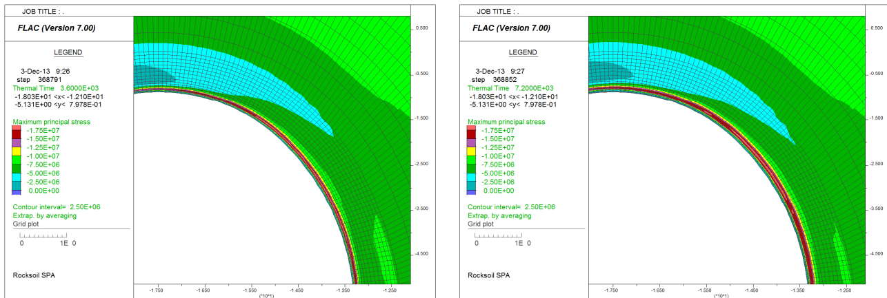
Figura 61 – Sigma 1 – Curva UNI11076 – t = 120 min
