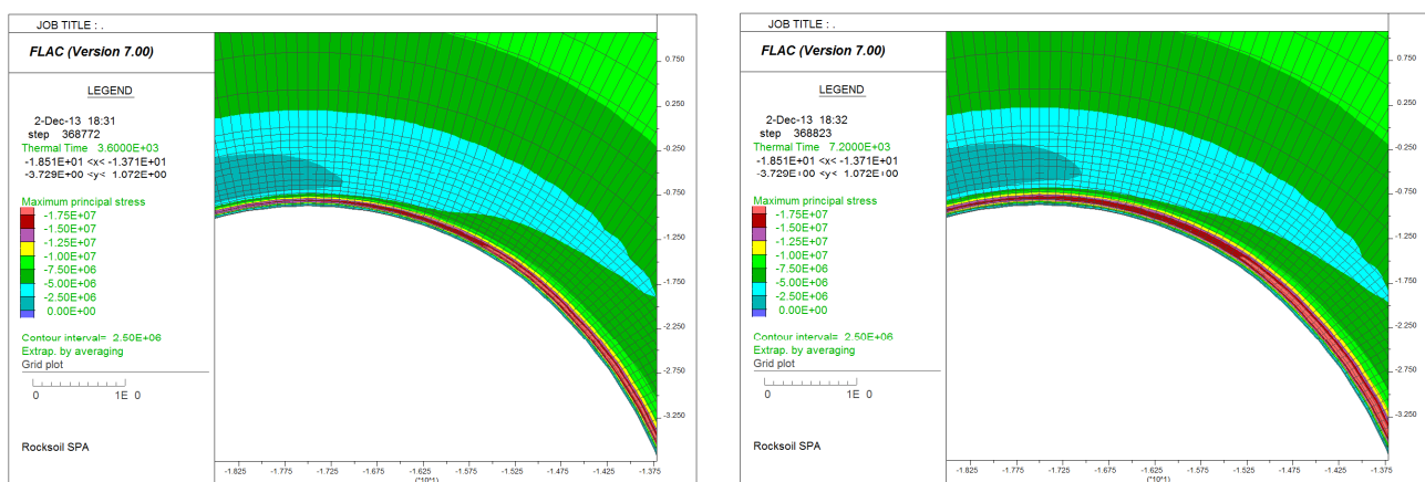
Figura 60 – Sigma 1 – Curva EUREKA – t = 120 min
