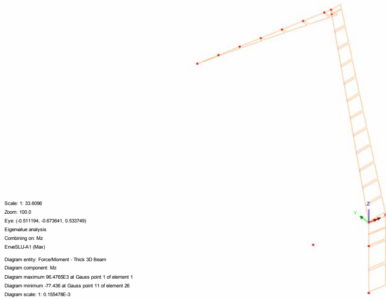
Fig. 31 – Mz (Local)
