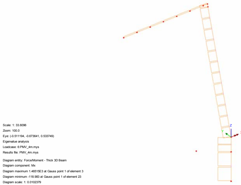
Fig. 29 – Mx (Local) - Buffeting L1
