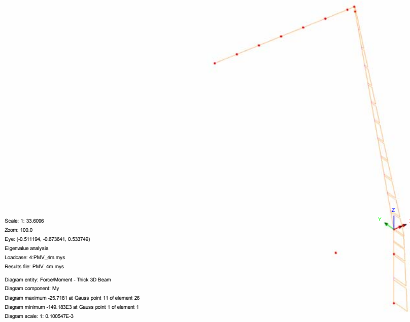
Fig. 20 – My (Local) - Vento
