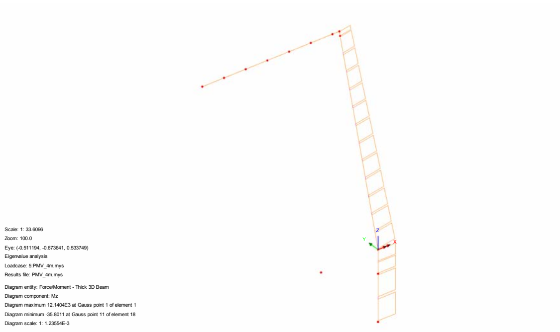
Fig. 24 – Mz (Local) - Neve
