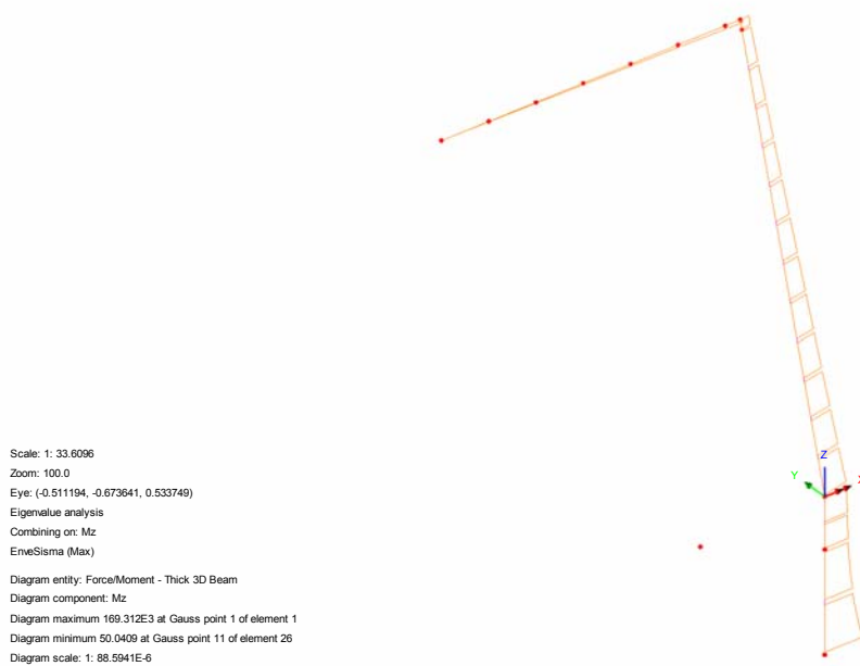
Fig. 37 – Mz (Local)
