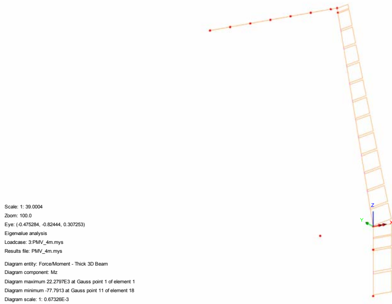
Fig. 19 – Mz (Local) - Permanenti portati
