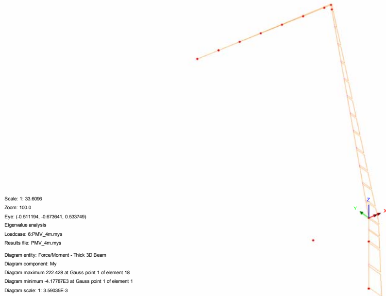
Fig. 27 – My (Local) - Buffeting L1
