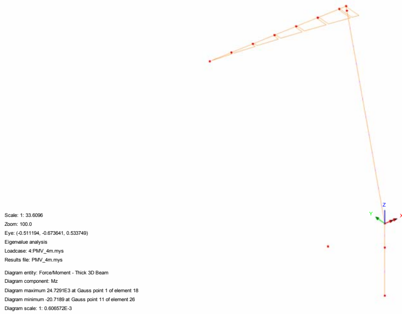
Fig. 21 – Mz (Local) - Vento
