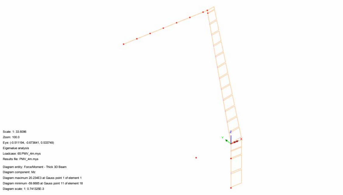
Fig. 26 – Mz (Local) - Folla
