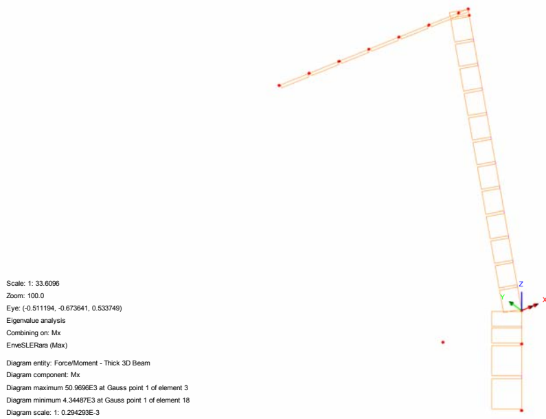
Fig. 35 – Mx - Torcente (Local)
