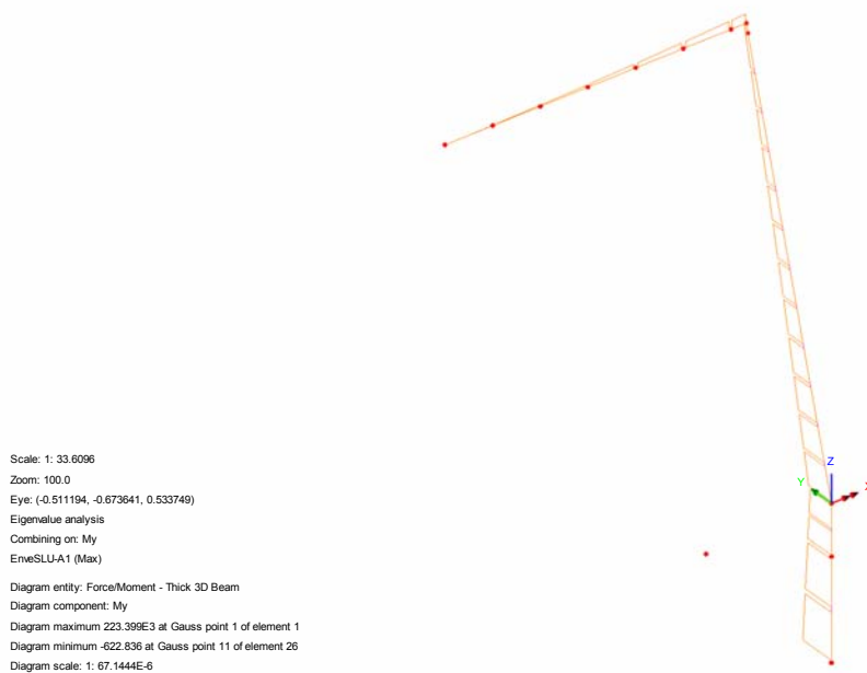
Fig. 30 – My (Local)
