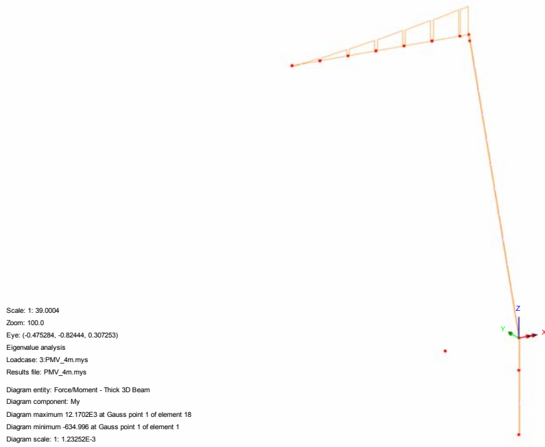
Fig. 18 – My (Local) - Permanenti portati
