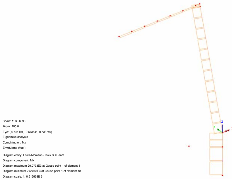
Fig. 38 – Mx - Torcente (Local)
