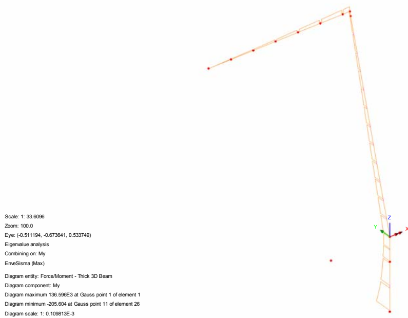
Fig. 36 – My (Local)
