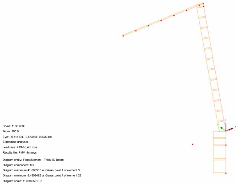
Fig. 22 – Mx - Torcente (Local) - Vento
