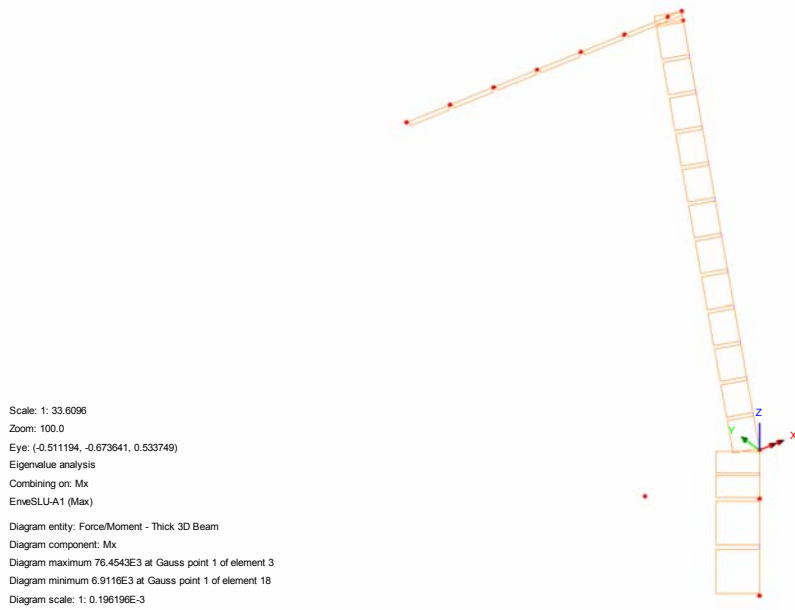
Fig. 32 – Mx - Torcente (Local)
