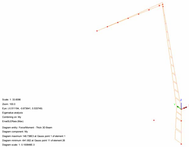
Fig. 33 – My (Local)
