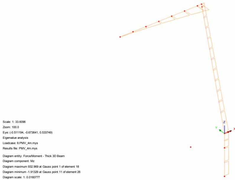
Fig. 28 – Mz (Local) - Buffeting L1
