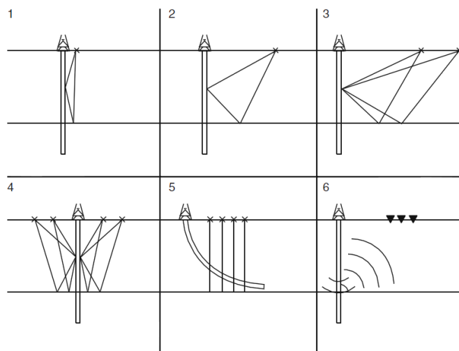
Vertical Seismic Profiling: Common acquisition geometries for vertical seismic profiling (VSP): (1) zero-offset VSP (ZVSP), (2) offset VSP, (3) multi-offset VSP, (4) walk-away VSP, (5) walk-above VSP, and (6) drill-bit SWD (seismic while drilling) VSP.
