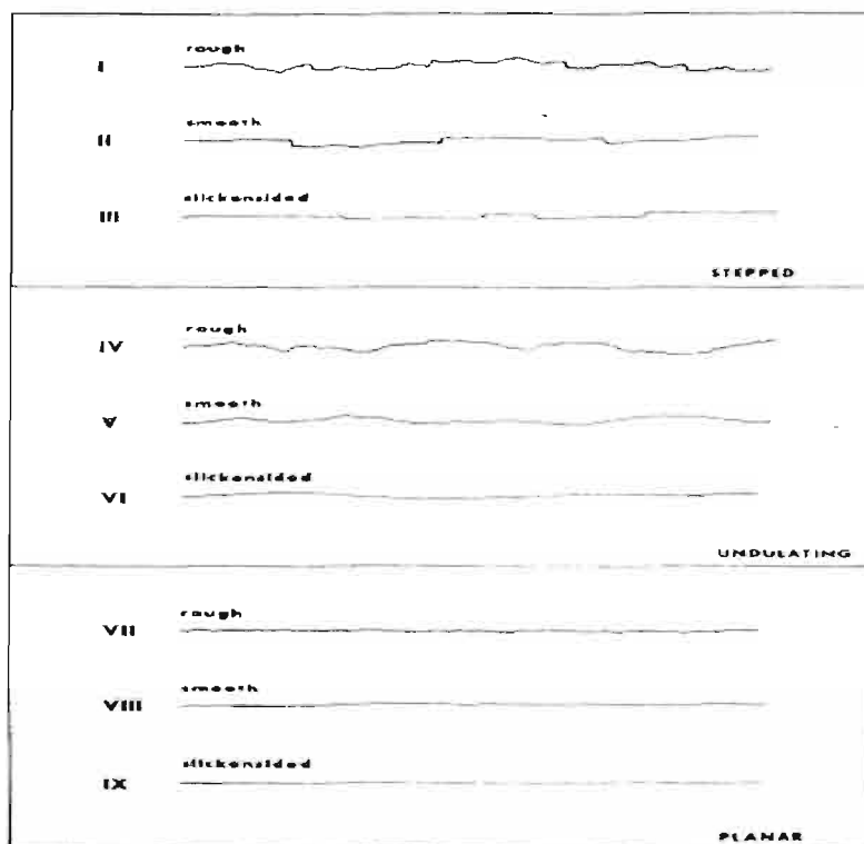
Fig.9 (ISRM, 1978)
