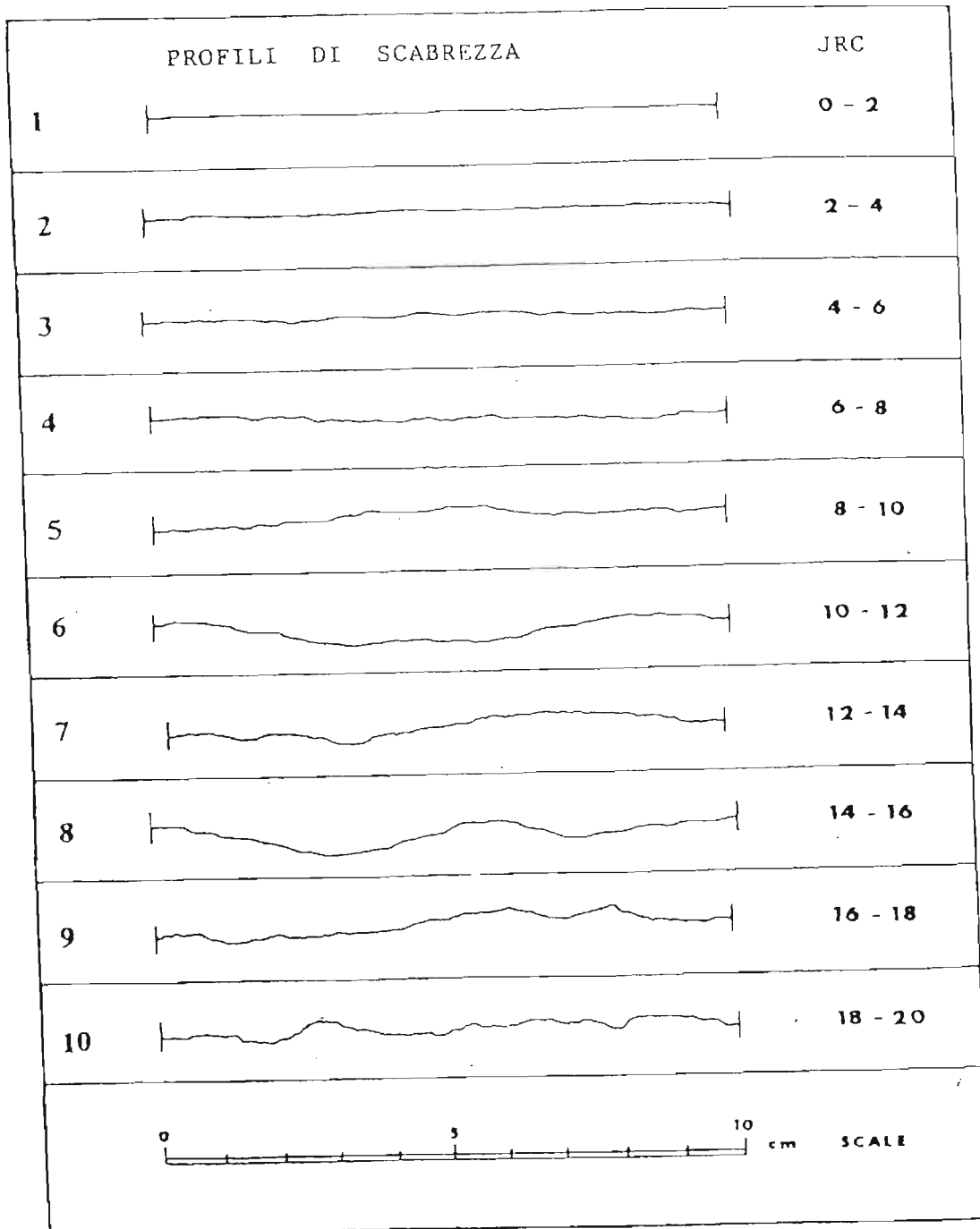
Fig.8a (Barton, 1974)
