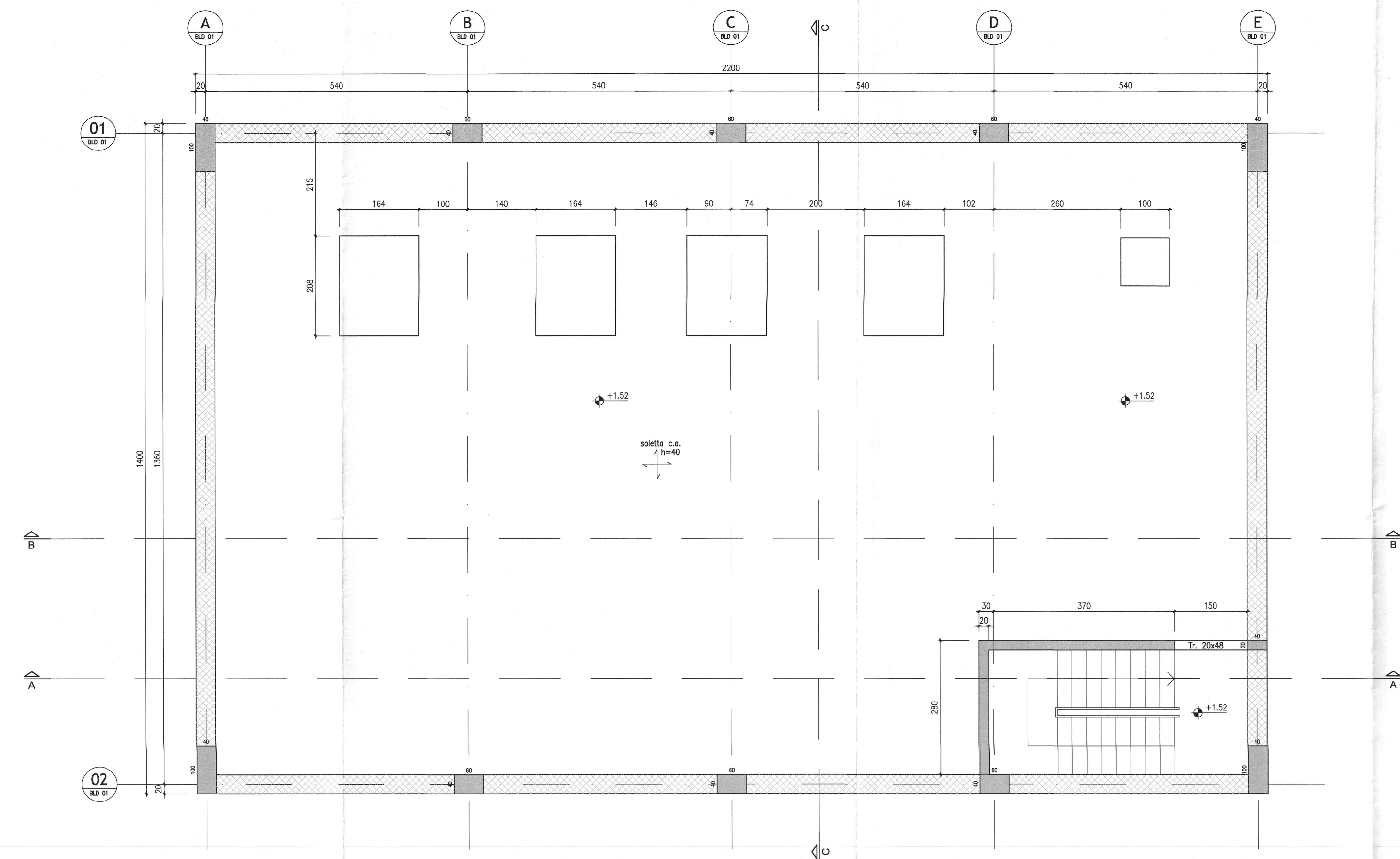
Carpenteria piano terra Q.ta +1.50 Scala 1:50
