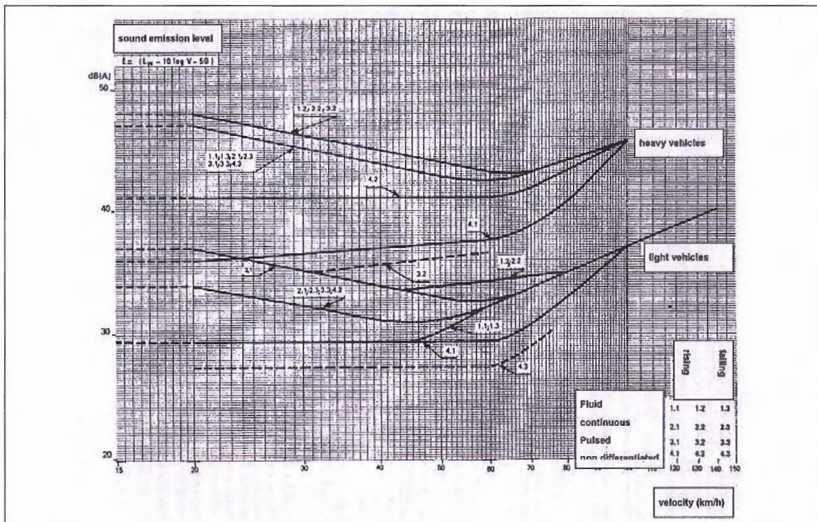
Figura 4.1 – Nomogramma NMPB
