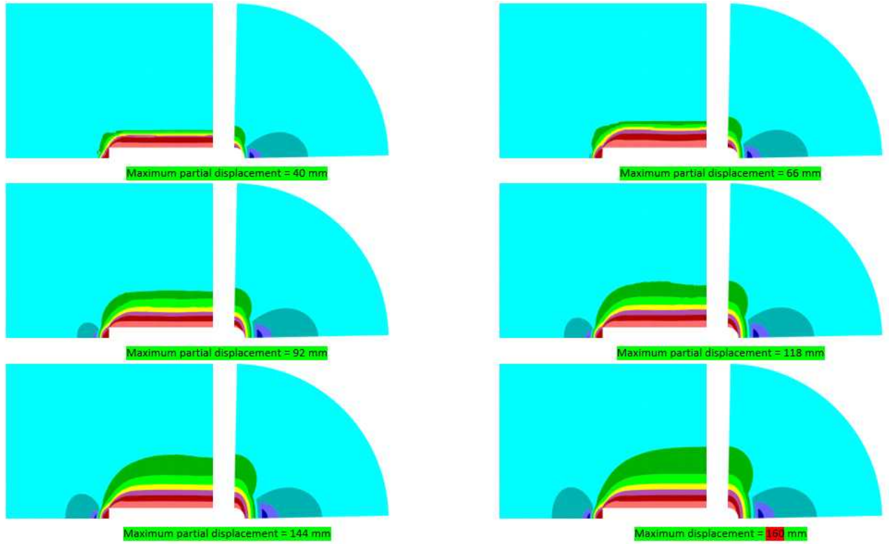
Contours of vertical stress corresponding to the maximal displacements, as indicated in the previous figure. The left side of each subfigure corresponds to the axisymmetrical model, whereas the right side to the plane strain model
