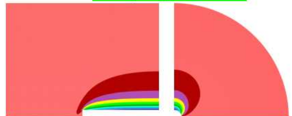
Contours of the development of vertical displacement of the exploratory tunnel at section K42 at six steps, for which the maximal partial displacement is given. The left side of each subfigure corresponds to the axisymmetrical model, whereas the right side to the plane strain model
