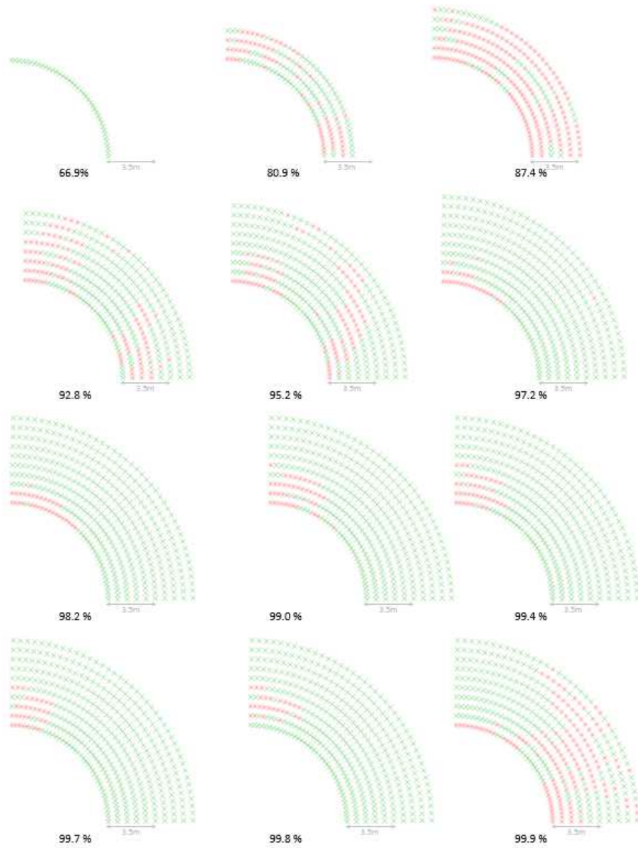
Development of the plasticized zone for the cross section of the excavation at different values of stress relaxation. Green color is used for those points currently under elastic behavior, but had been previously at yield. Red means points, which are currently at yield condition.
