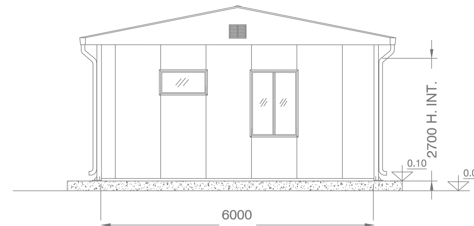
VISTA D)
