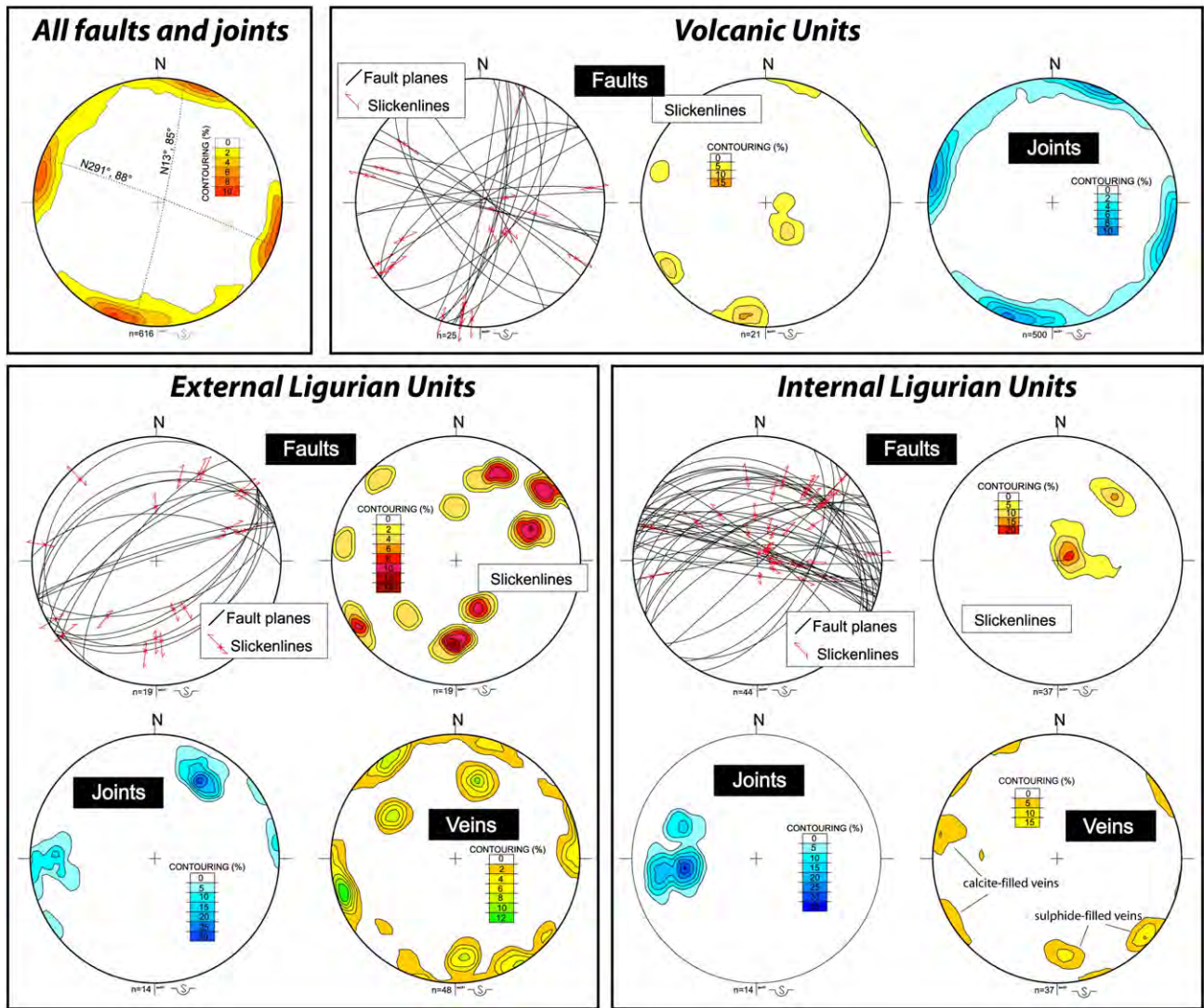
Fig. 4. Stereographic projections (Schmidt net, lower hemisphere) of the data collected in Ligurian (both internal and external) and volcanic units.
