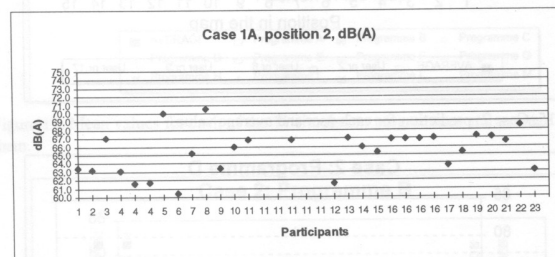
Fig. 18: Lmed = 65.5 dB(A) Lmax - Lmin = 10.1 dB(A) Std.Dev. = 2.47
