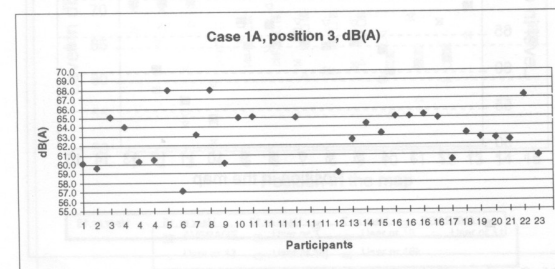
Fig. 19: Lmed = 63.1 dB(A) Lmax - Lmin = 10.9 dB(A) Std.Dev. = 2.69
