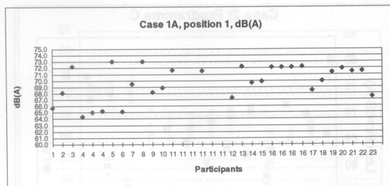
Fig. 17: Lmed = 69.7 dB(A) Lmax - Lmin = 8.7 dB(A) Std.Dev. = 2.66
