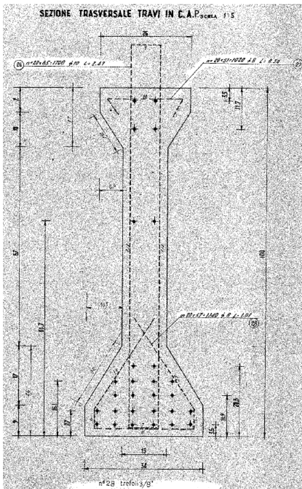
Trave – Campate unica
