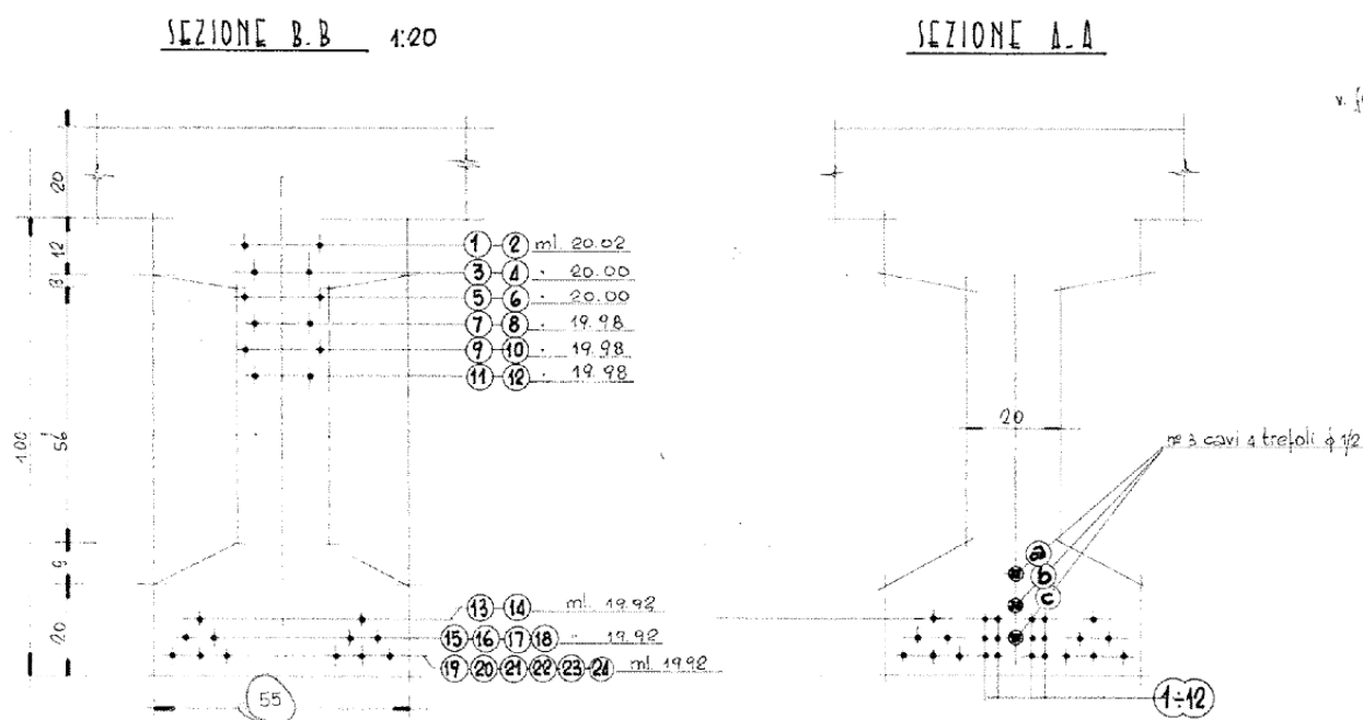
Trave – Campate unica
