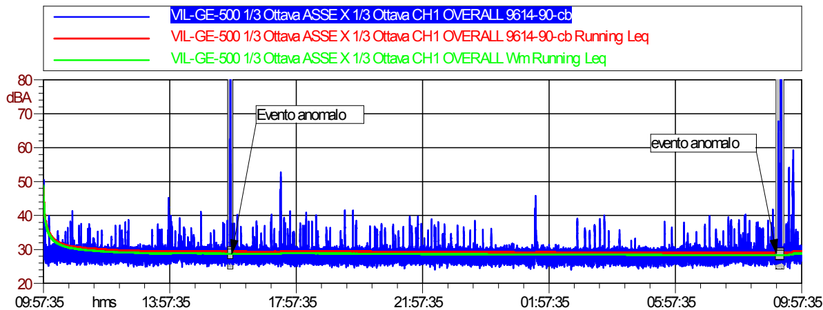
Figura 4.8.7 Time-History Asse X VIL-GE-500
