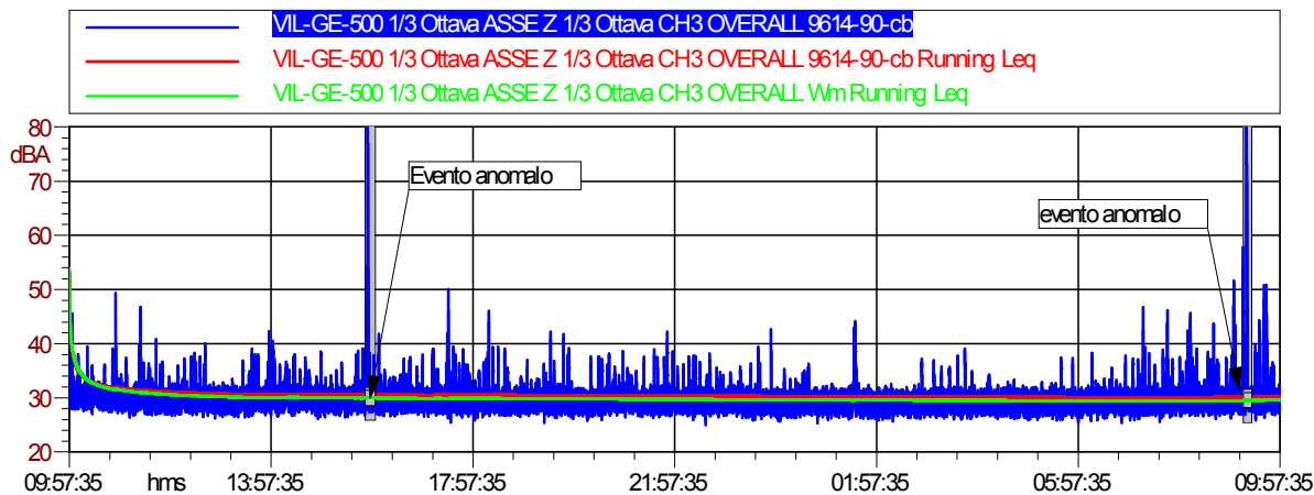
Figura 4.8.9 Time-History Asse Z VIL-GE-500
