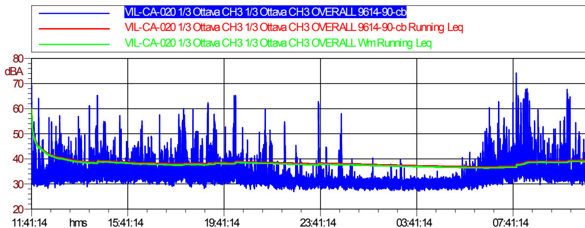
Figura 4.5.9 Time-History Asse Z VIL-CA-020
