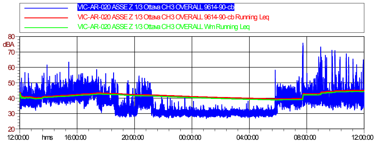
Figura 4.7.5 Time-History Asse Z
