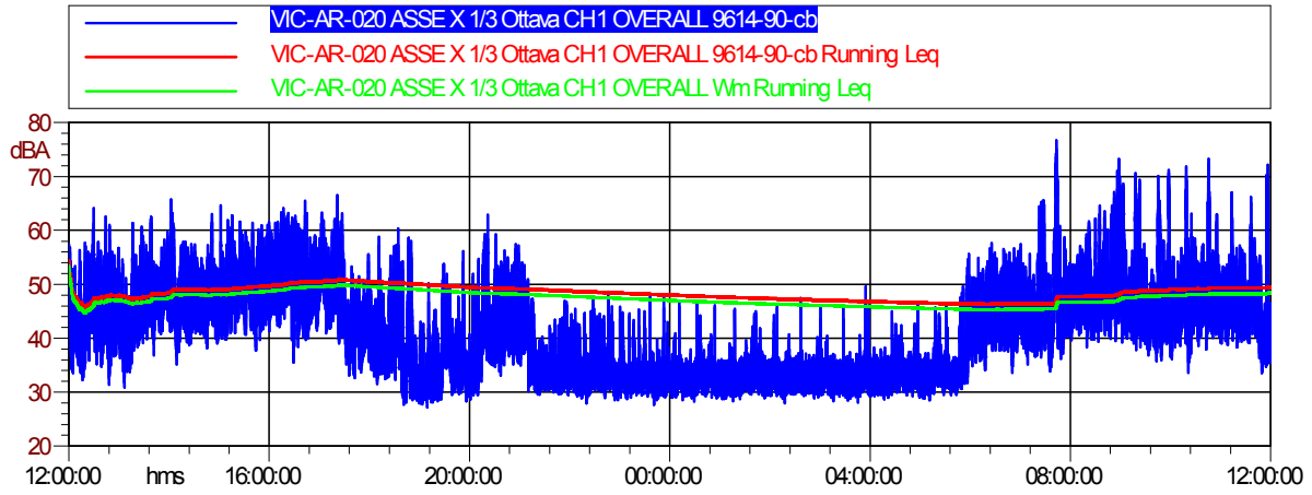
Figura 4.7.3 Time-History Asse X
