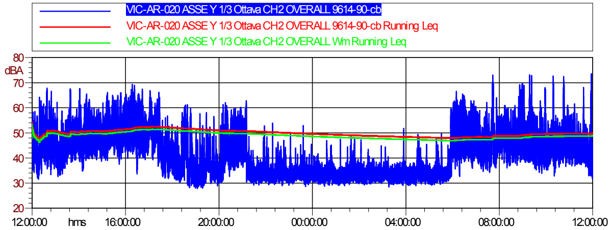
Figura 4.7.4 Time-History Asse Y
