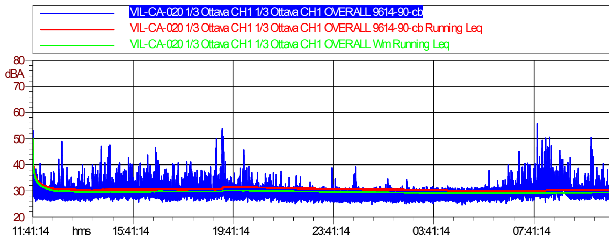
Figura 4.5.7 Time-History Asse X VIL-CA-020
