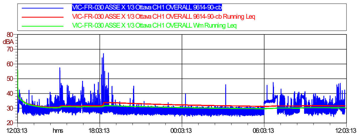
Figura 4.2.6 Time-History Asse X
