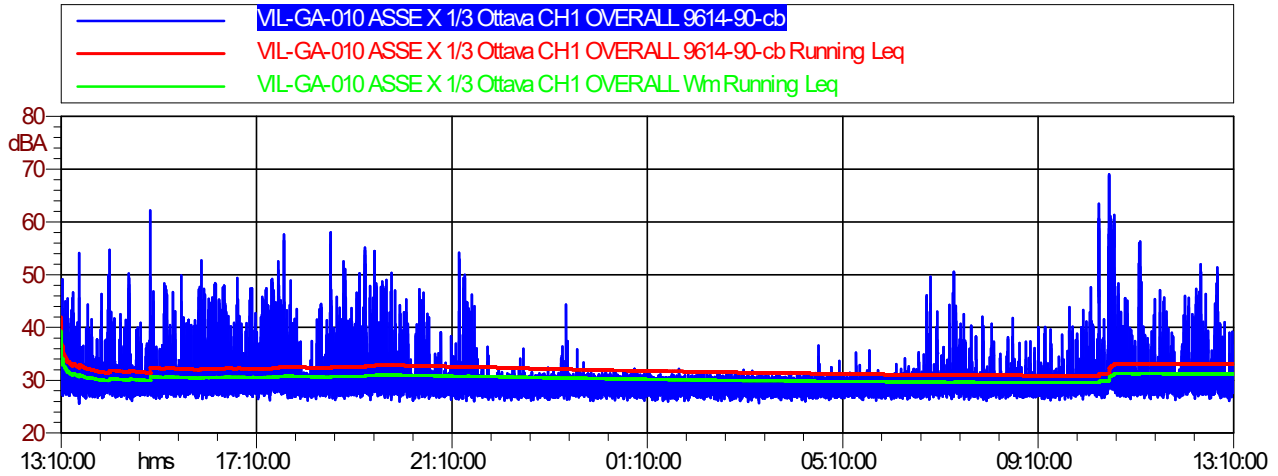
Figura 4.5.7 Time-History Asse X VIL-GA-010
