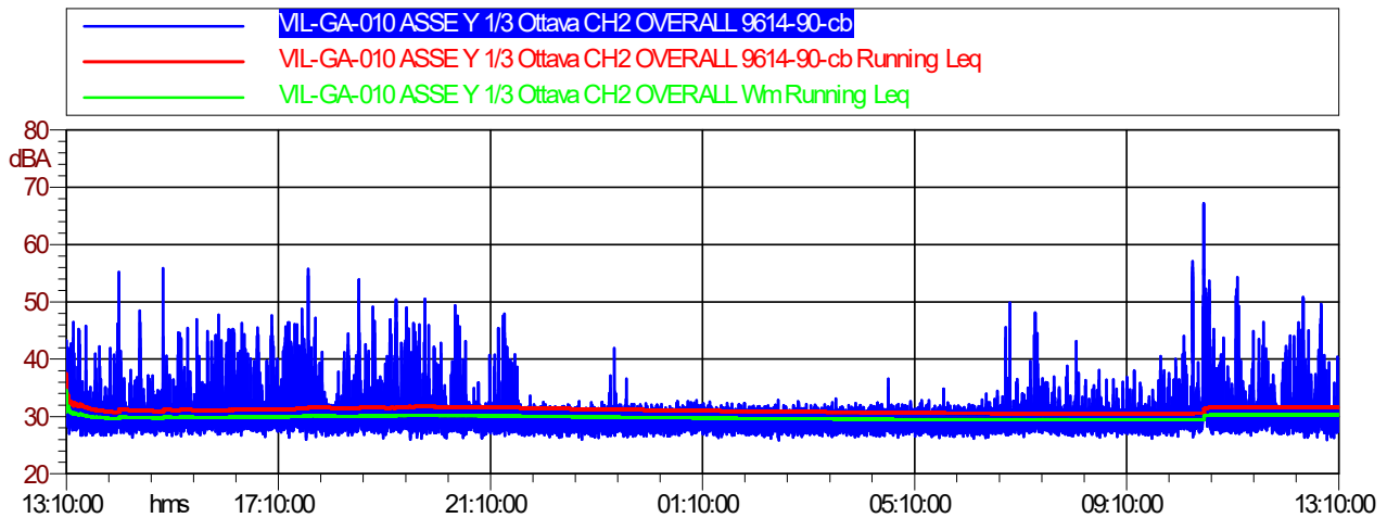
Figura 4.5.8 Time-History Asse Y VIL-GA-010
