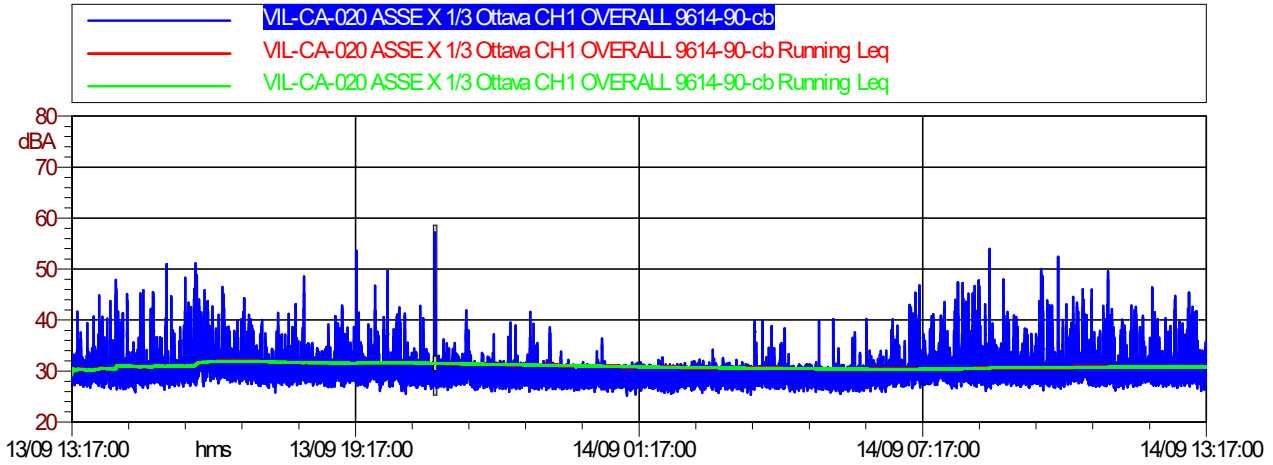
Figura 4.5.7 Time-History Asse X VIL-CA-020
