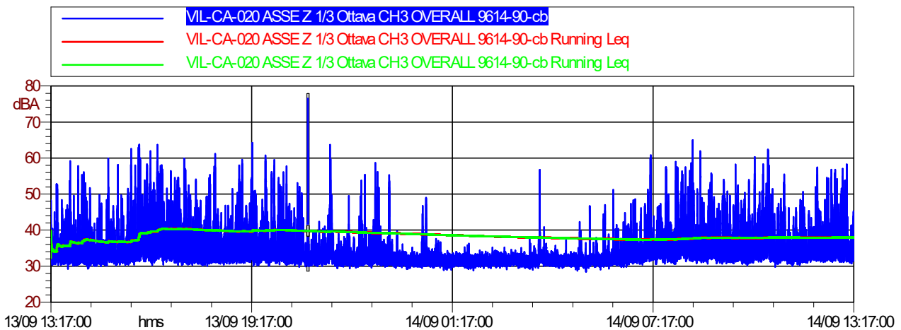
Figura 4.5.9 Time-History Asse Z VIL-CA-020
