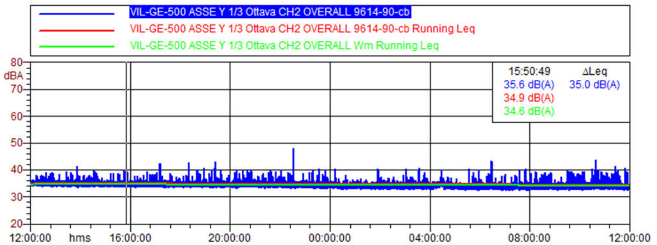
Figura 4.8.8 Time-History Asse Y VIL-GE-500
