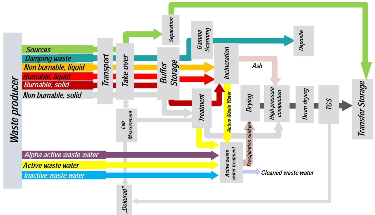
Figure 4: Material flow of radioactive waste treatment in NES
