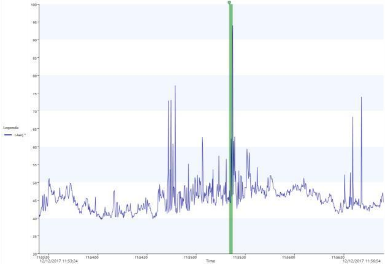
Figura 22 - Misura1: Time history
