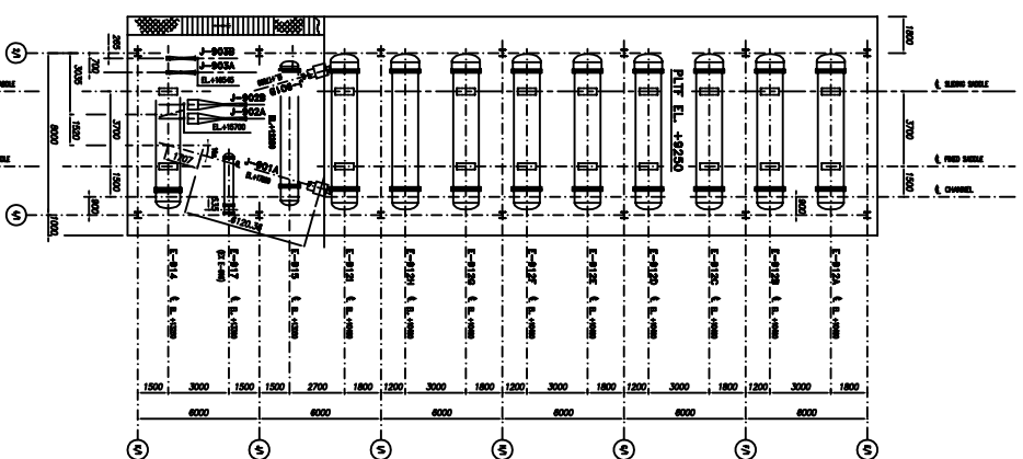
PLAN AT EL. +9250
