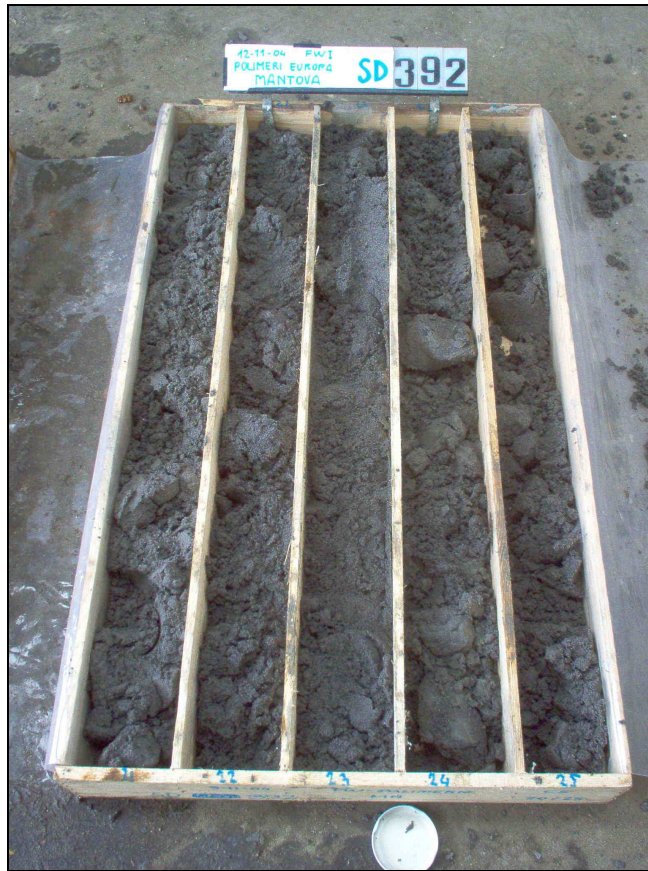
SD392: 20.00-25.00m
