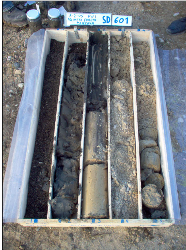
SD601: 0.00-5.00m
