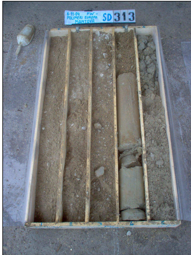
SD313: 0.00-5.00m
