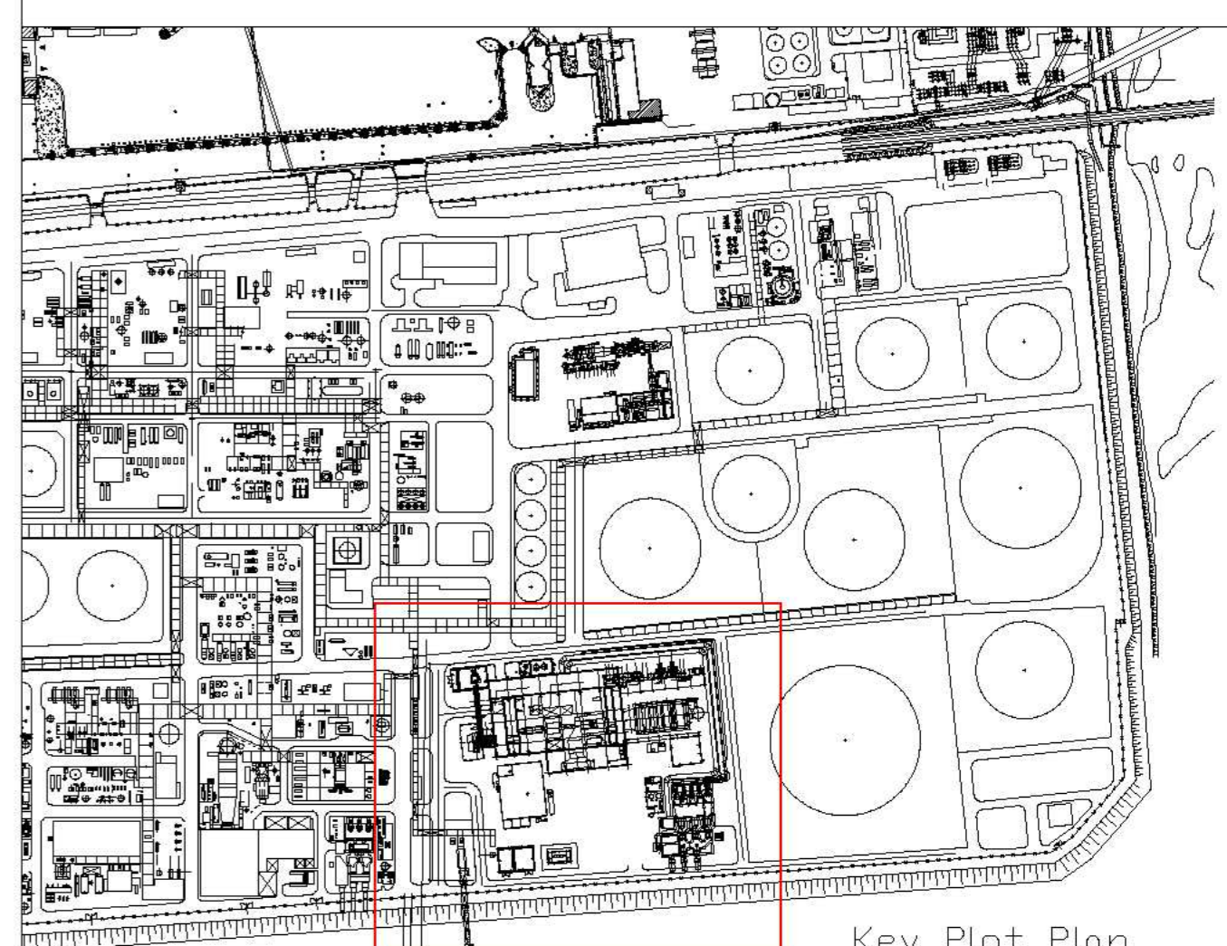
Key Plot Plan
