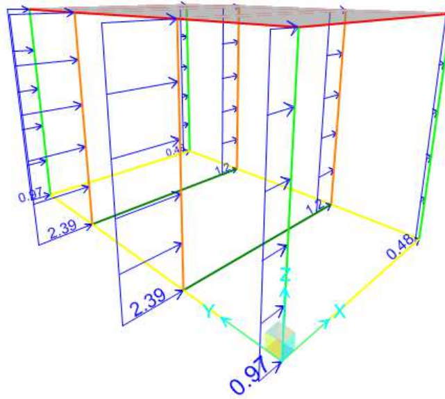
Frame Span Loads (Vy) (GLOBAL CSys)
