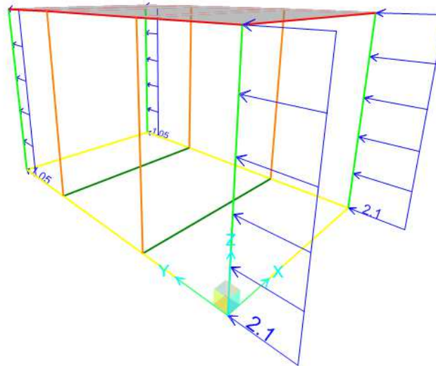
Frame Span Loads (Vy) (GLOBAL CSys)
