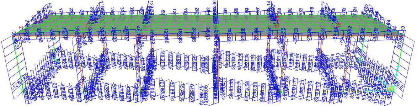
Shear Force 2-2 Diagram (ENV-SLV)
