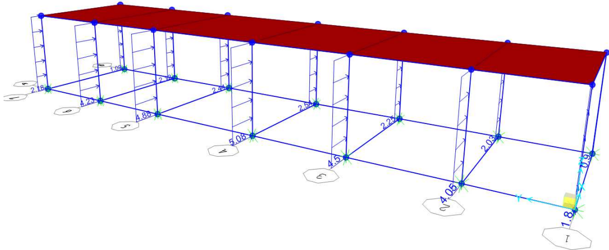
Frame Span Loads (Vx) (GLOBAL CSys)
