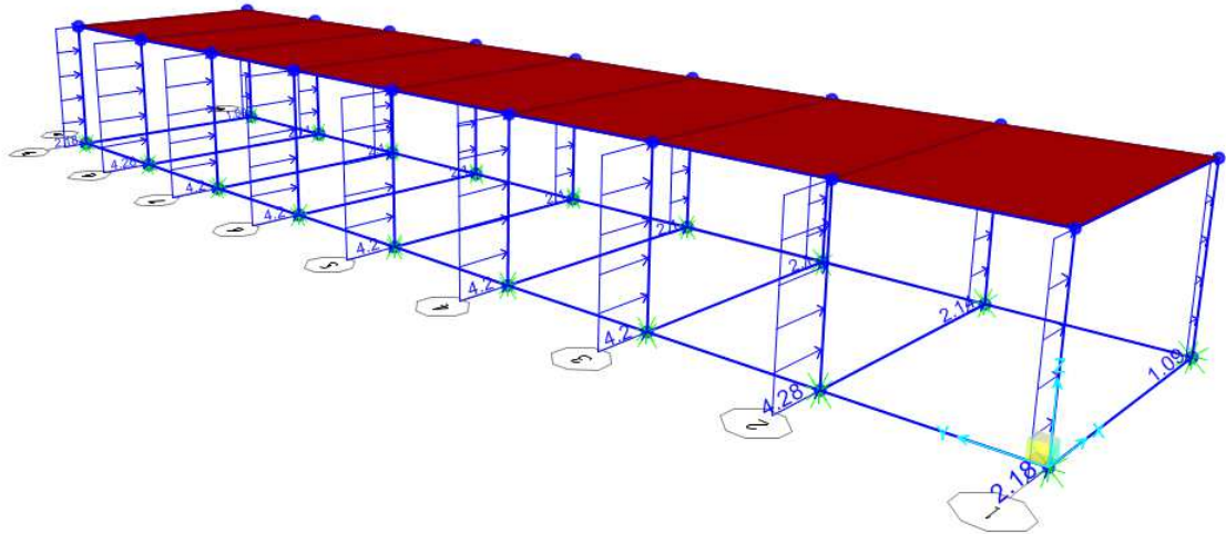
Frame Distributed Loads (Vy)
