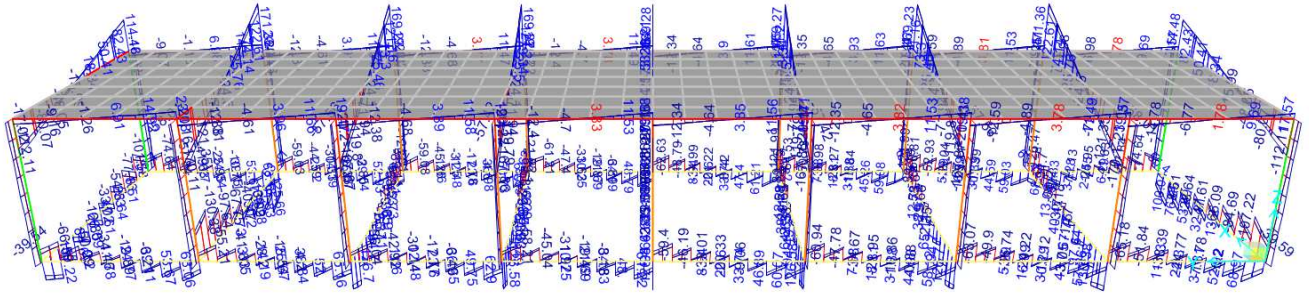
Shear Force 2-2 Diagram (_ENV-SLU)
