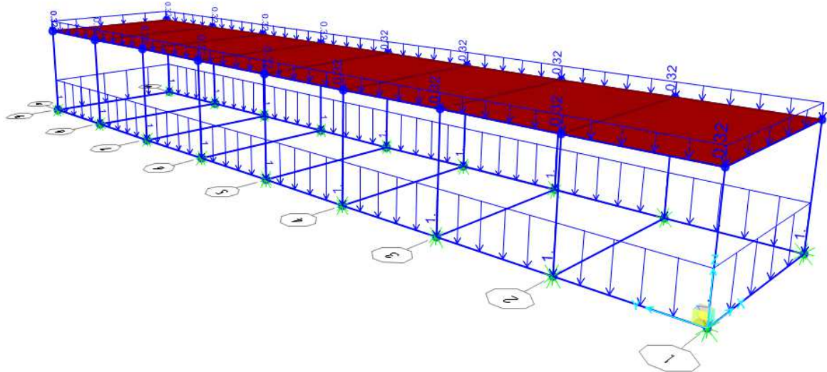
Frame Distributed Loads (G2k_M)
