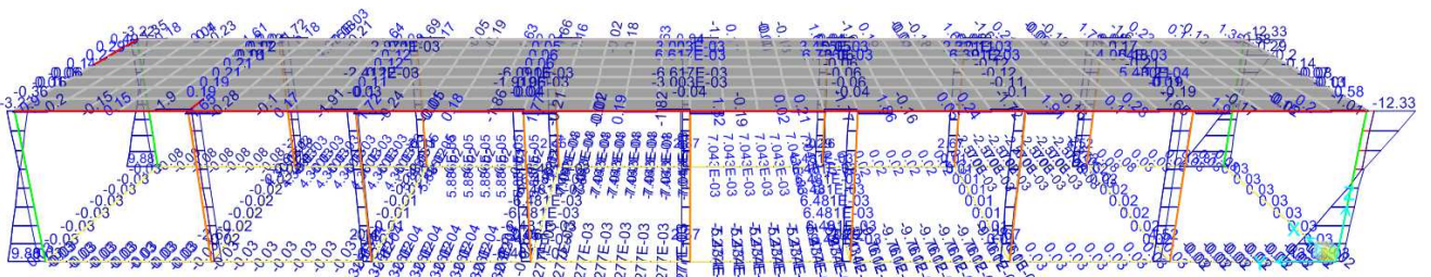
Shear Force 3-3 Diagram (_ENV-SLU)
