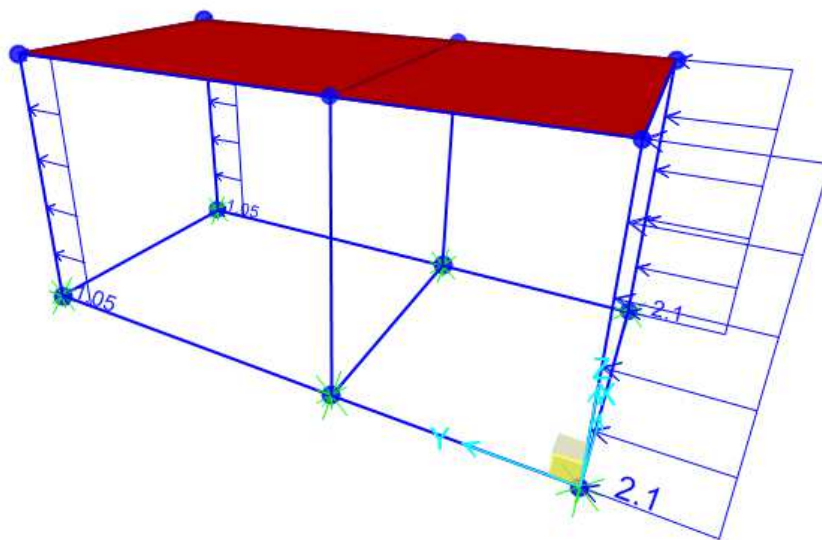
Frame Span Loads (Vy) (GLOBAL CSys)
