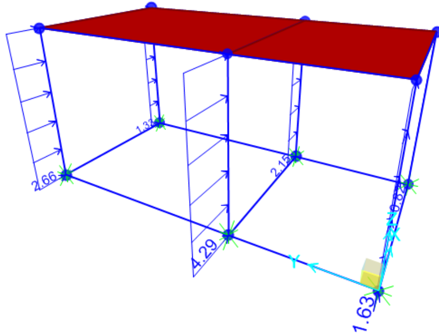
Frame Span Loads (Vy) (GLOBAL CSys)
