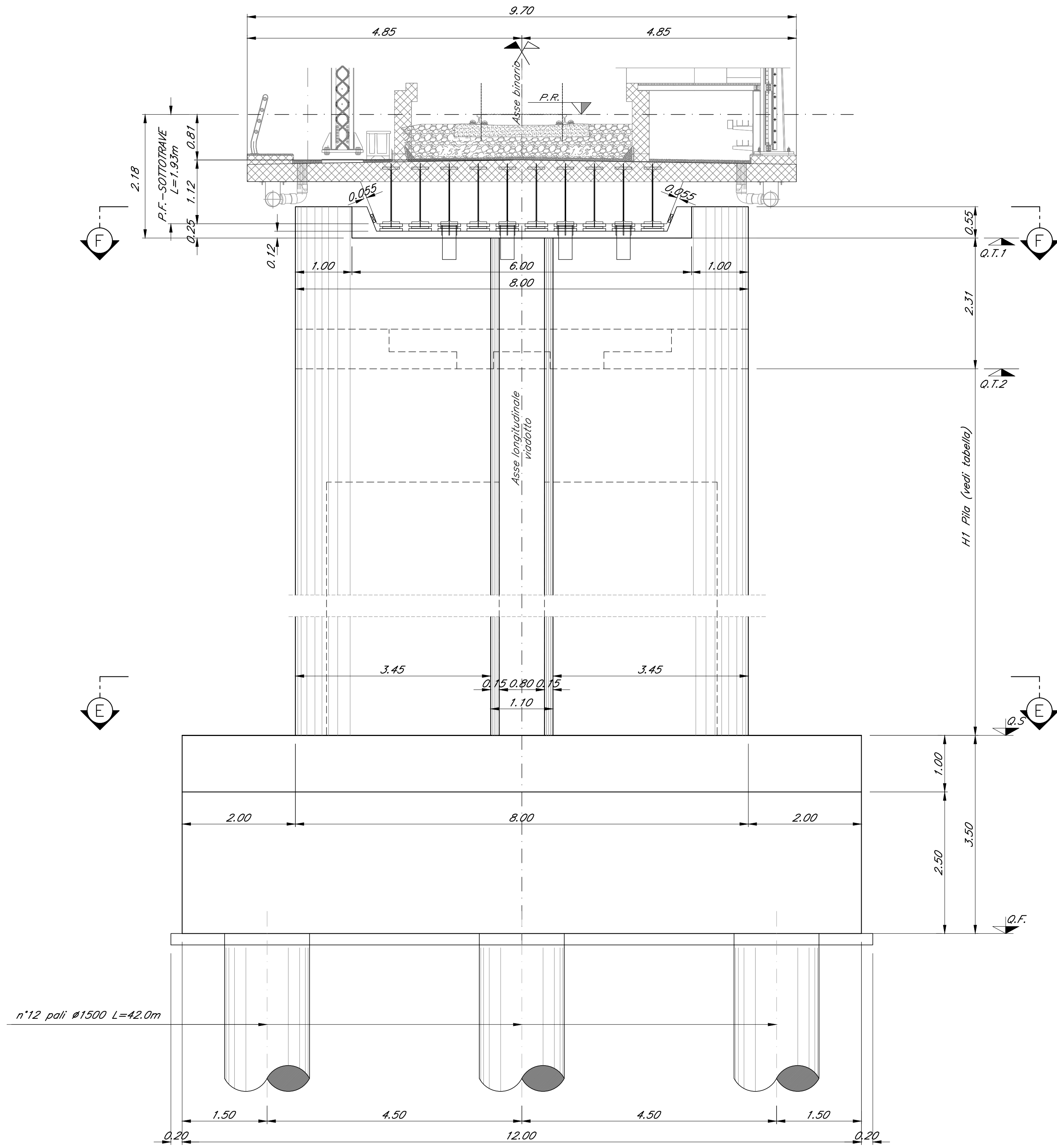
CARPENTERIA PILE P1 B.P. e P1 B.D. Scala 1:50
