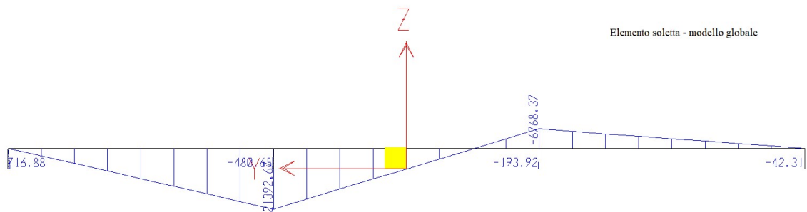
Moment 2-2 Diagram (12)
