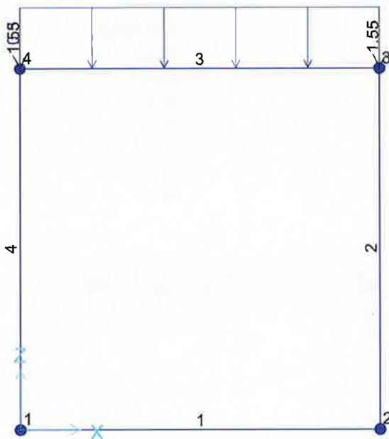
FIGURA 7-2: CARICHI PERMANENTI (PERM)
