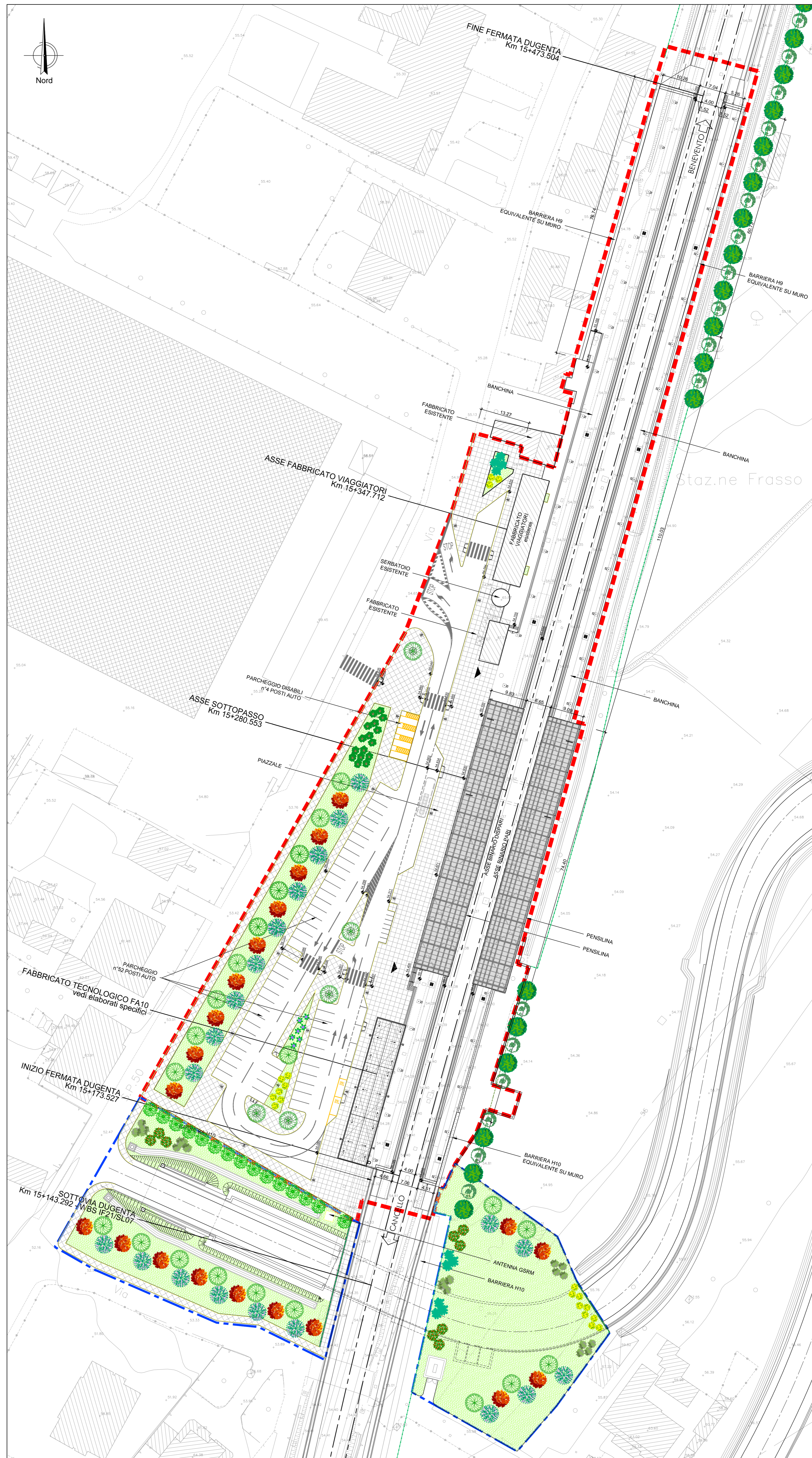
PLANIMETRIA POST OPERAM SCALA 1:500
