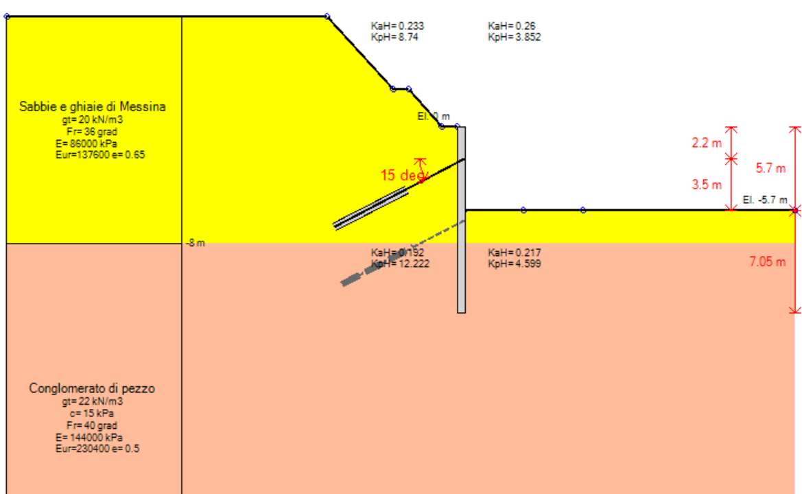
Stage 3 – Scavo a quota -5.70 m
