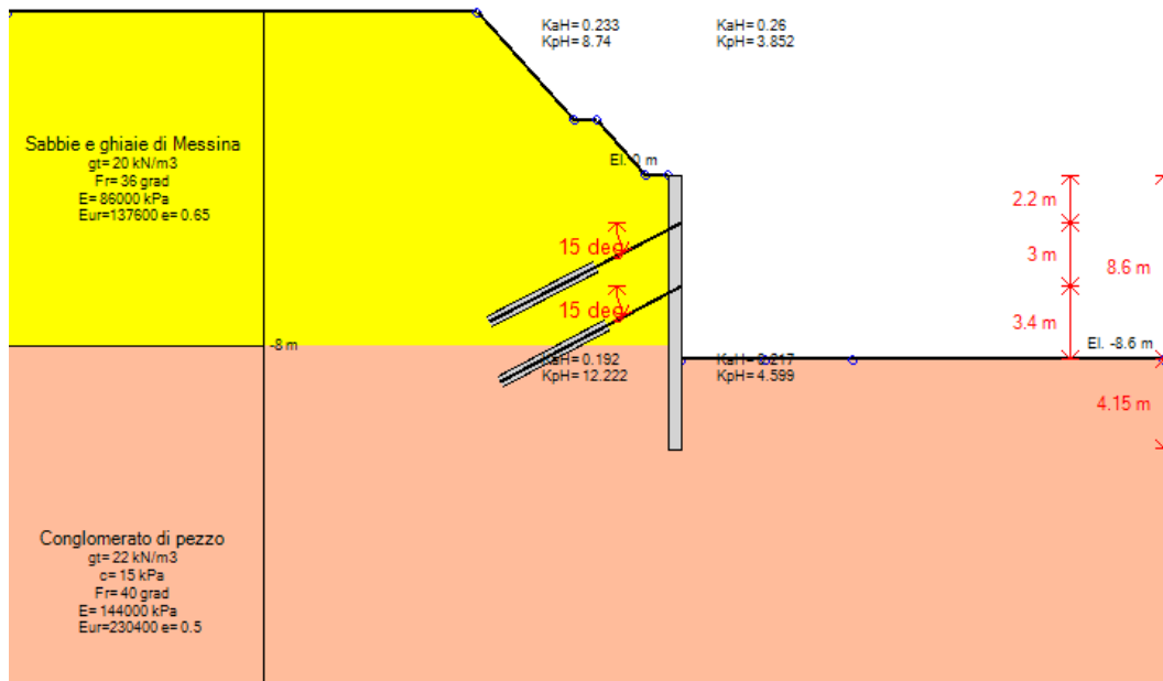
Stage 5 – Scavo a quota -8.60 m
