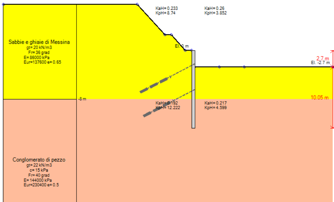
Stage 1 – Scavo a quota -2.70 m
