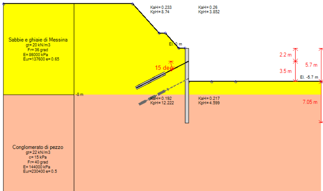
Stage 3 – Scavo a quota -5.70 m
