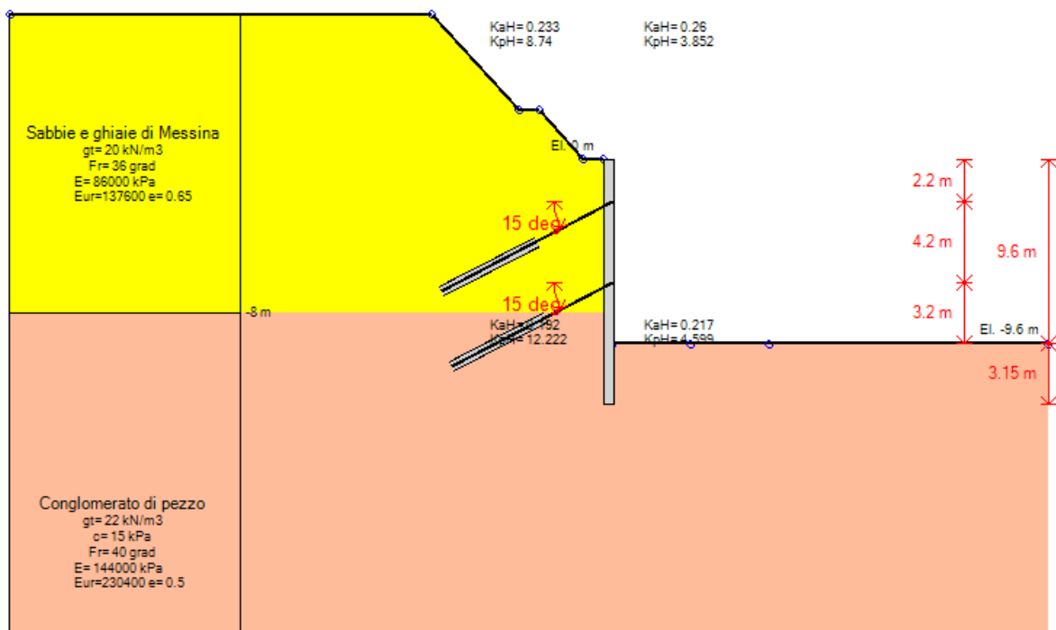
Stage 7 – Scavo a quota -9.60 m
