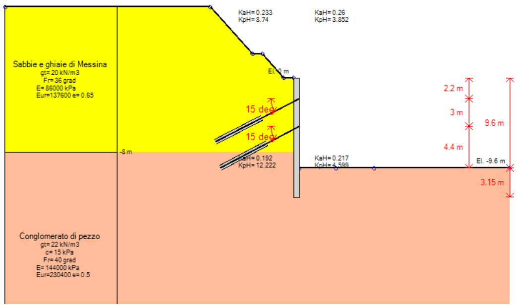
Stage 5 – Scavo a quota -9.60 m
