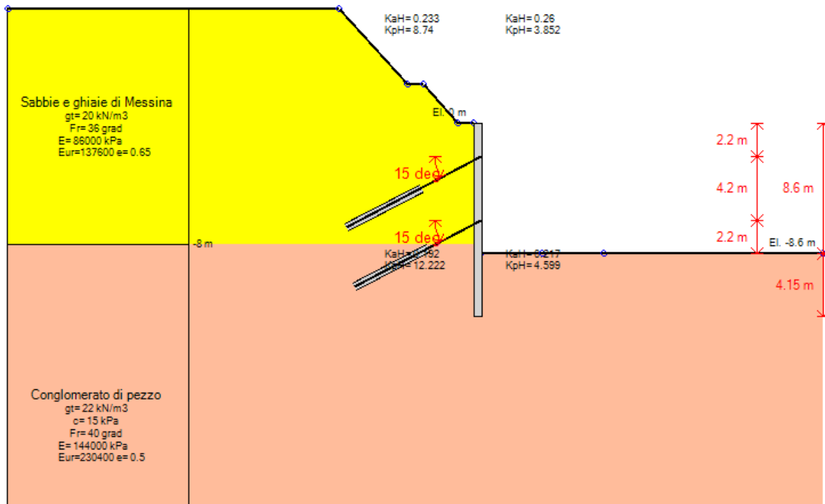
Stage 6 – Scavo a quota -8.60 m
