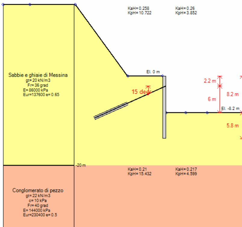
Stage 5 – Sisma
