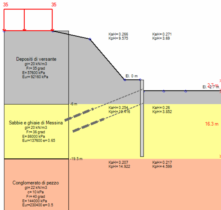
Stage 1 – Scavo a quota -2.70 m
