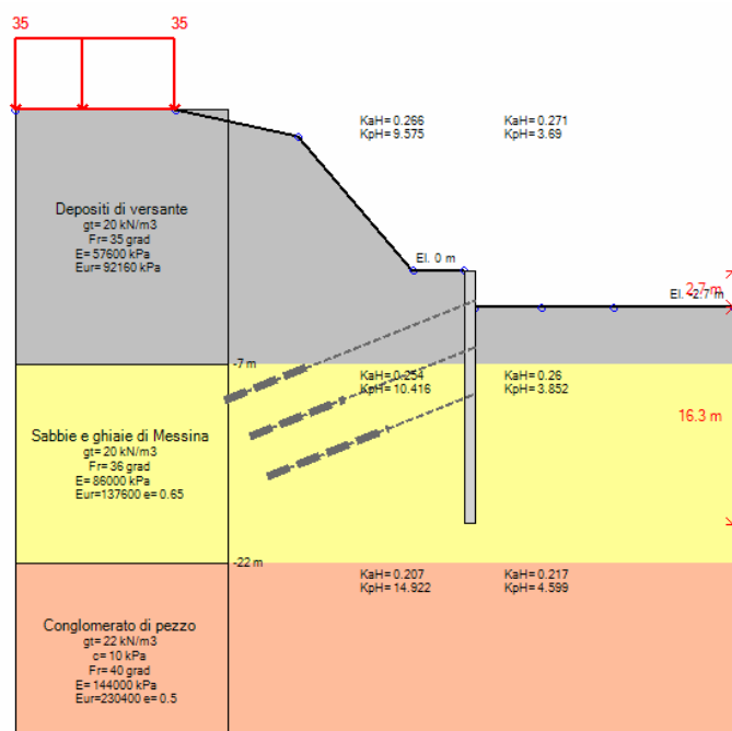
Stage 1 – Scavo a quota -2.70 m
