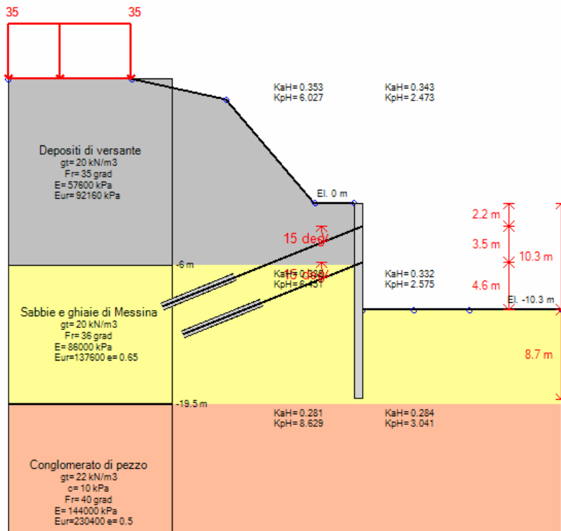
Stage 7 – Sisma
