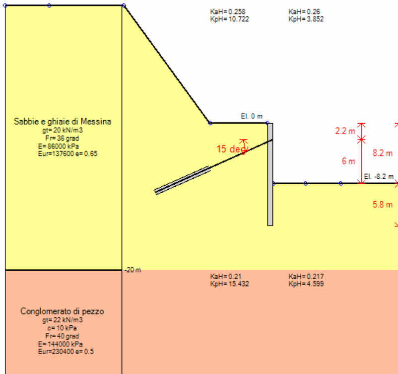
Stage 4 – Scavo a quota -8.20 m
