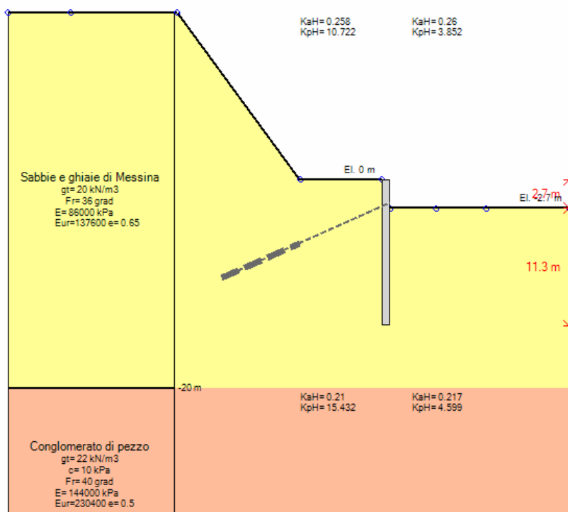
Stage 1 – Scavo a quota -2.70 m
