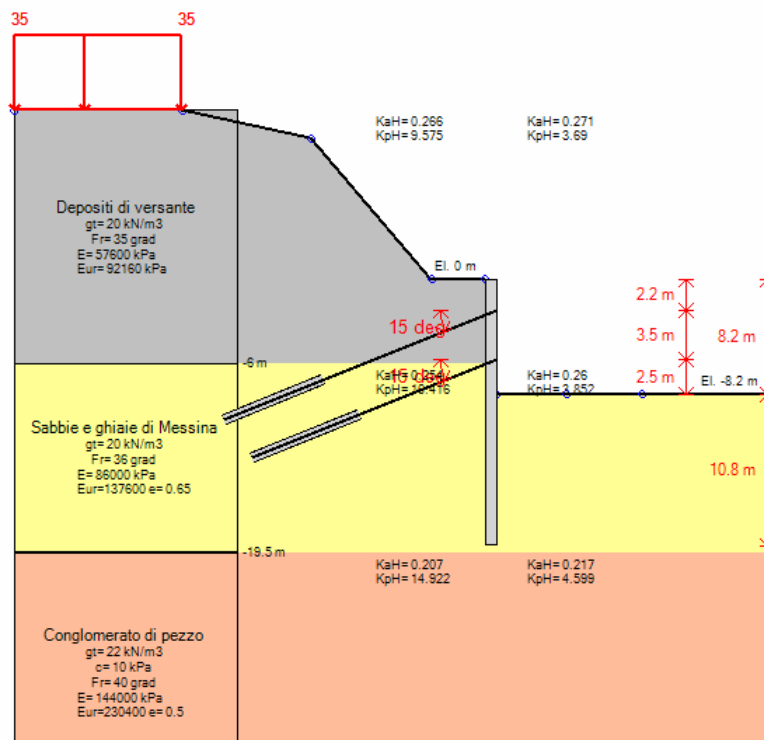
Stage 5 – Scavo a quota -8.20 m
