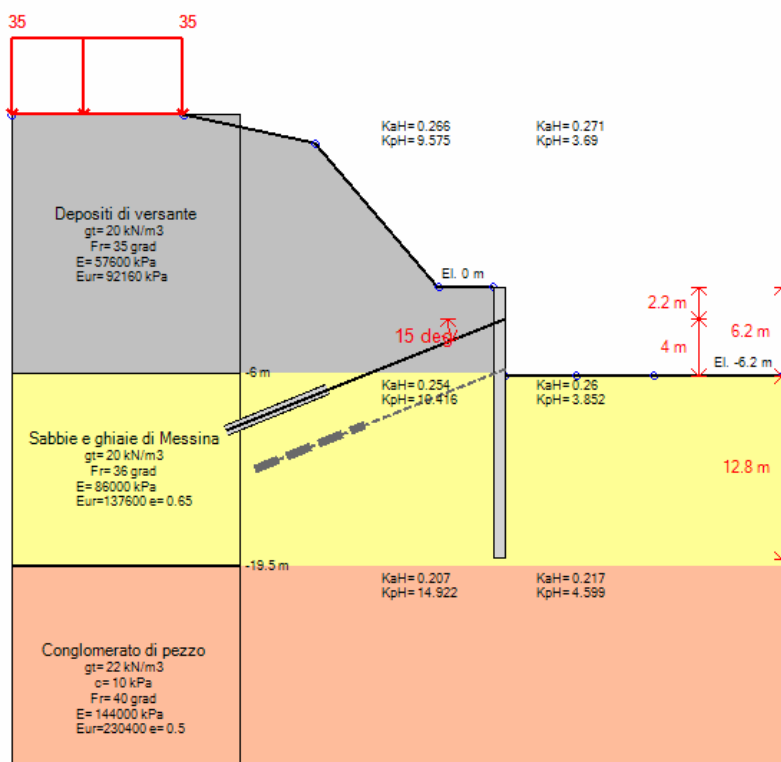
Stage 3 – Scavo a quota -6.20 m
