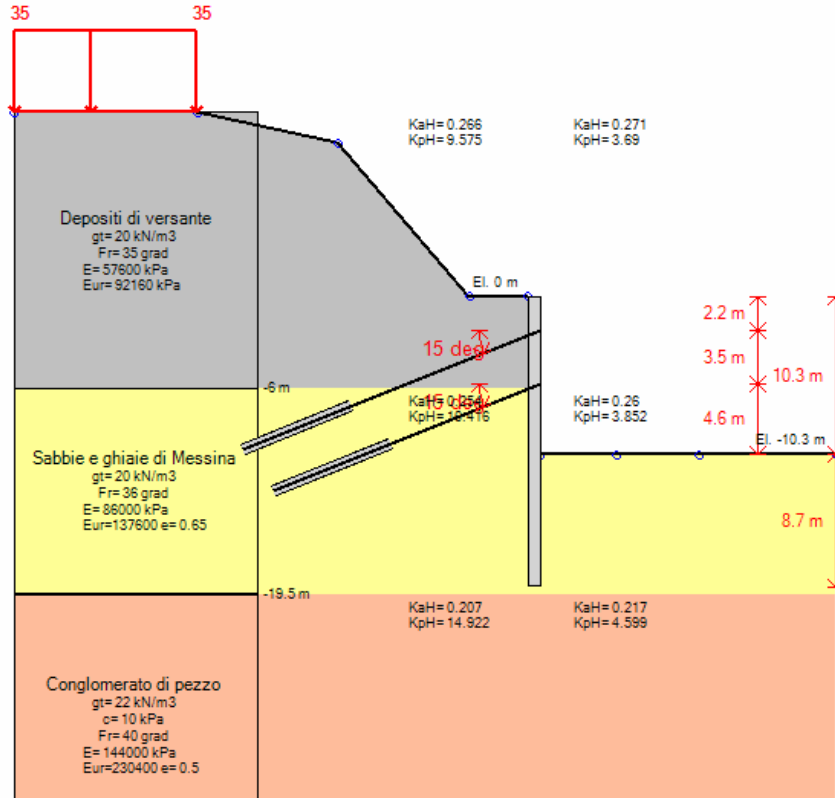
Stage 6 – Scavo a quota -10.30 m
