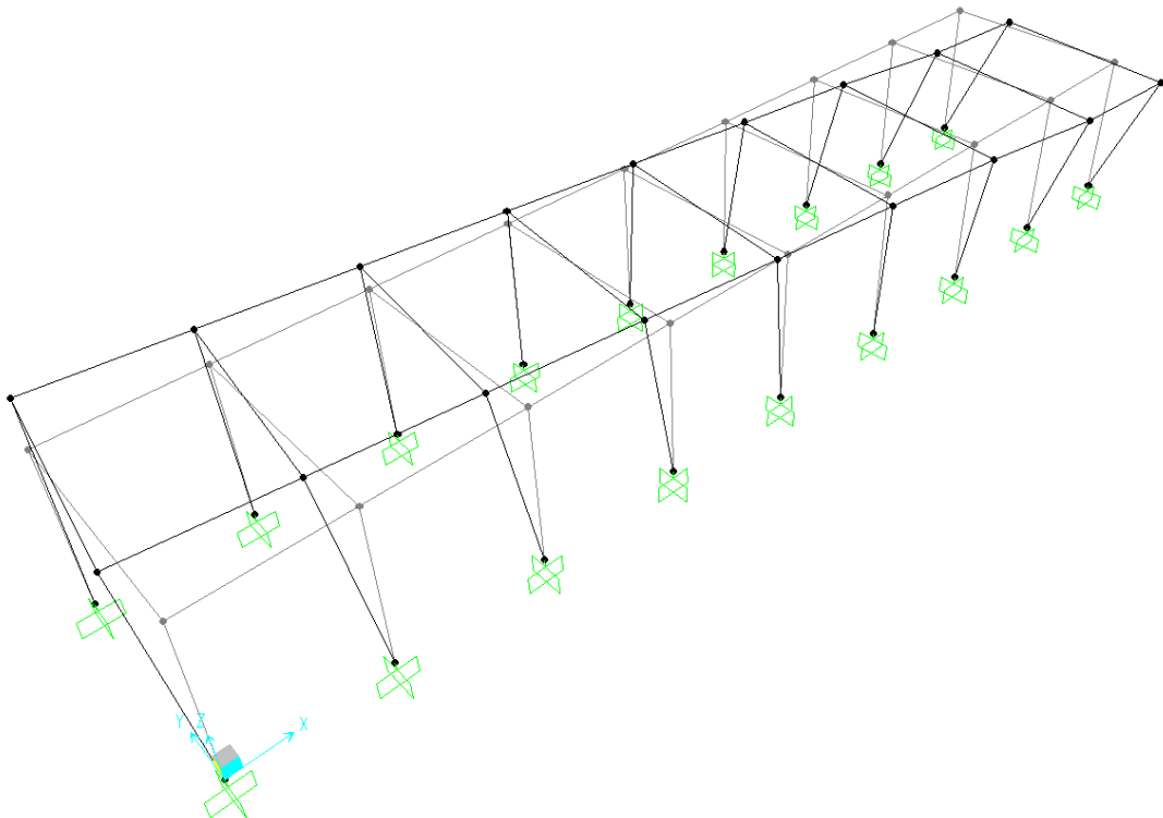
Deformed Shape (MODAL) - Mode 2 - Period 0.39305
