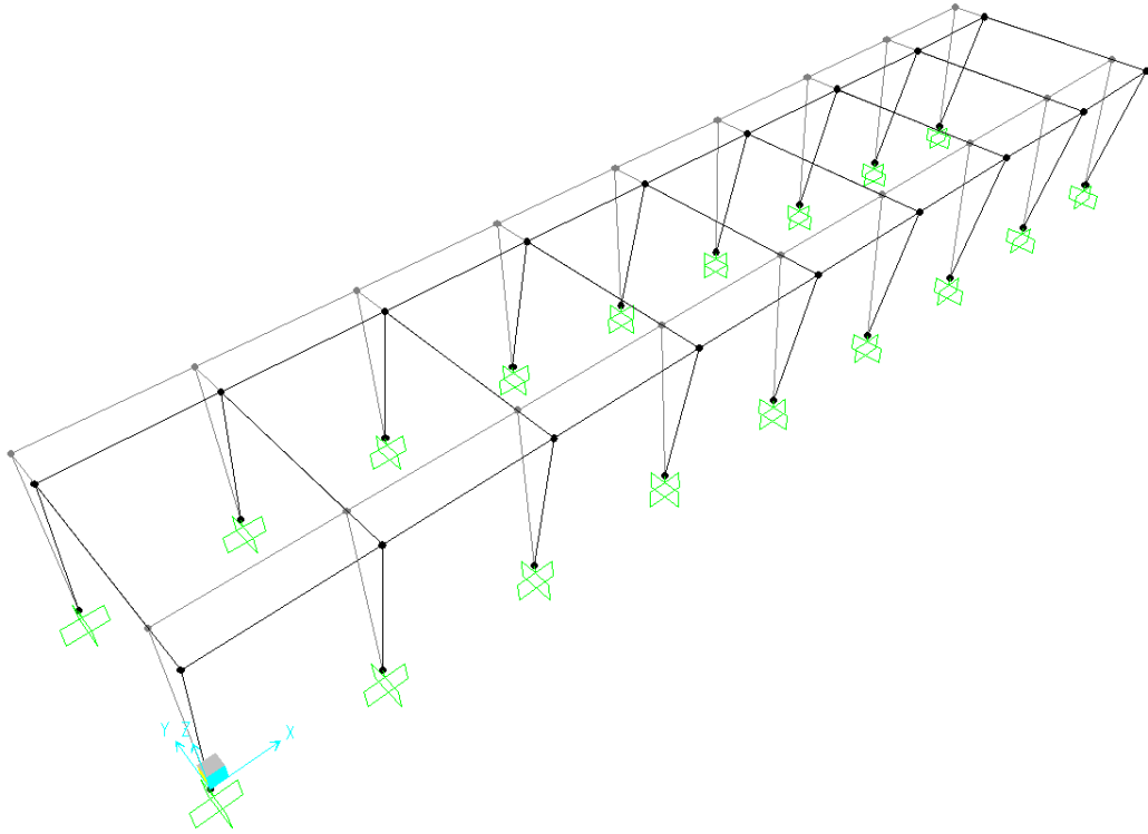
Deformed Shape (MODAL) - Mode 1 - Period 0.44414
