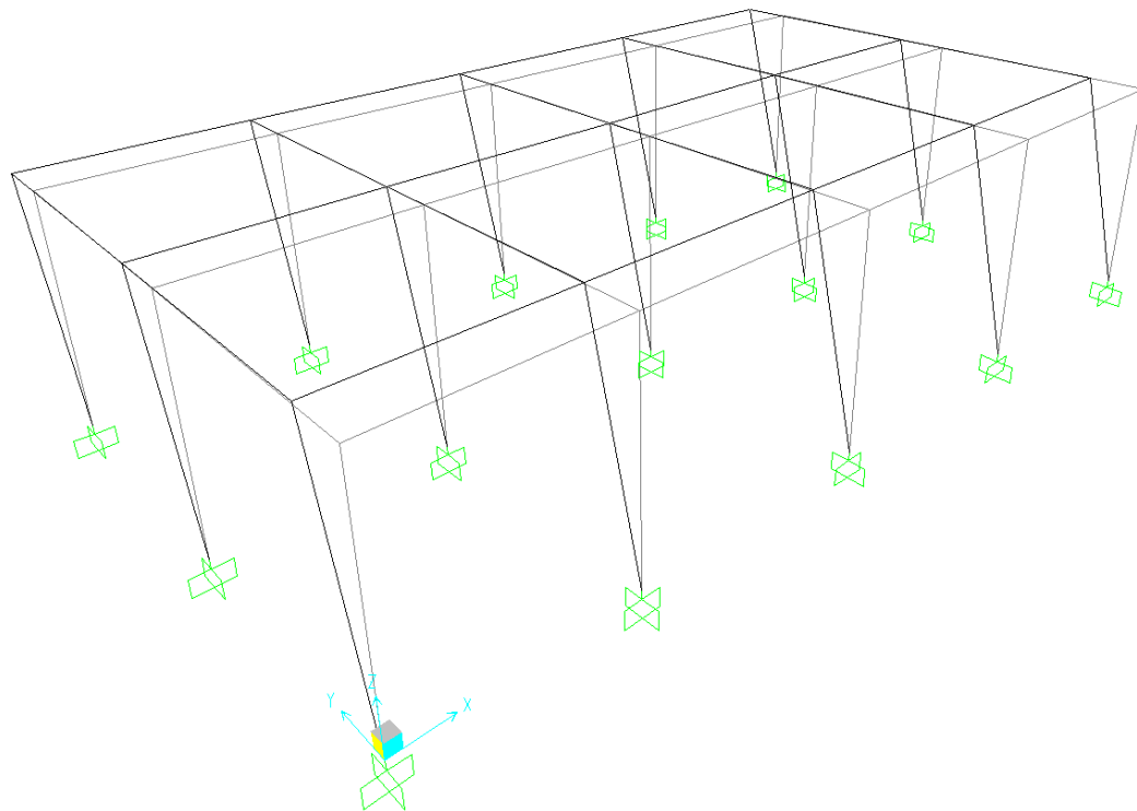
Deformed Shape (MODAL) - Mode 2 - Period 0.46775
