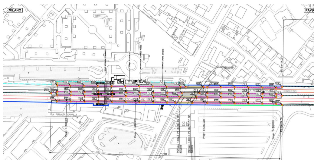
Figura 5 – Stralcio planimetrico elaborato NM0Z10D26P8FV010B001A
