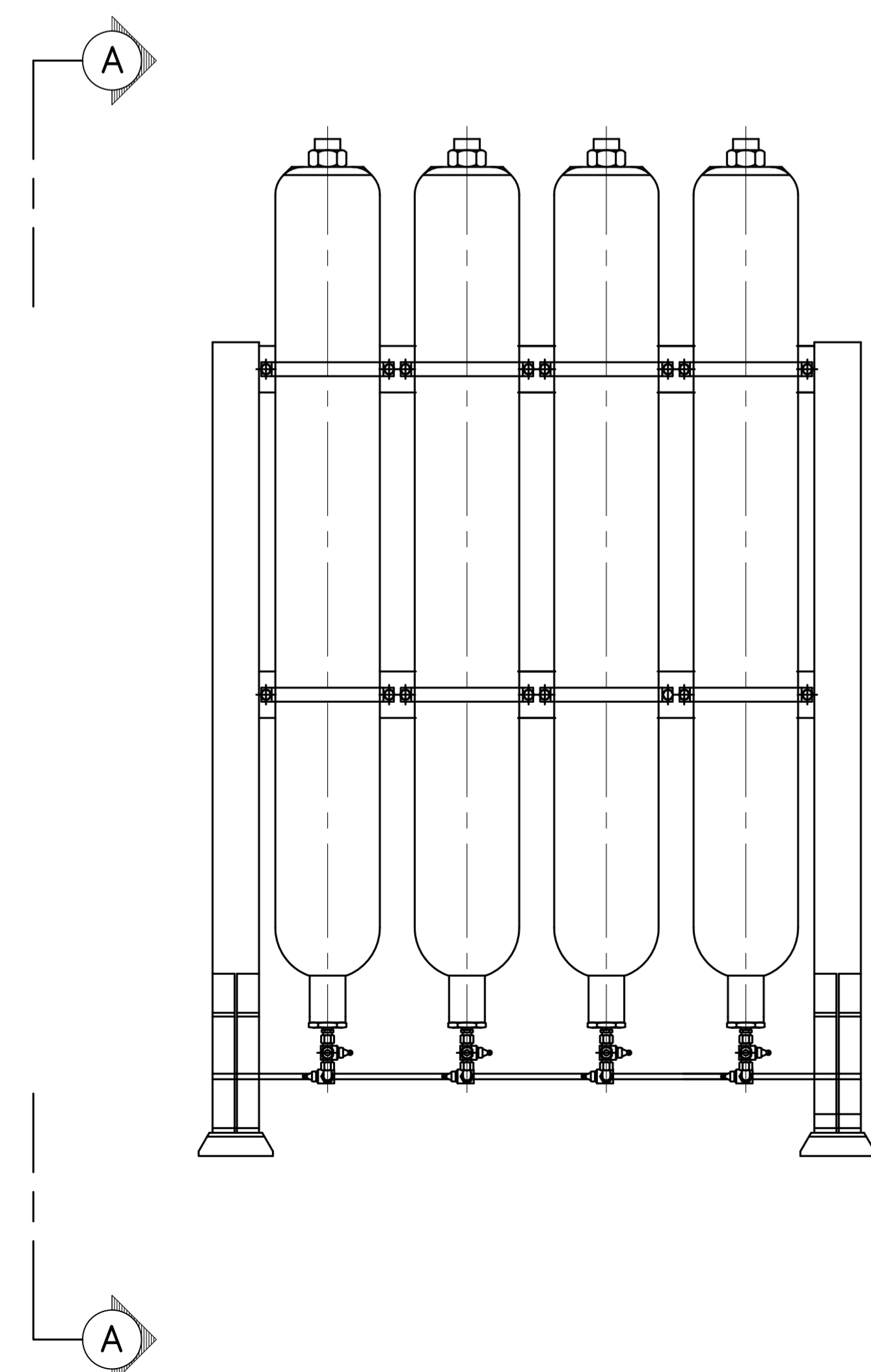
UNITA ACCUMULATORE PER BUFFER D2 NON IN SCALA ACCUMULATOR UNIT FOR BUFFER D2 NOT TO SCALE
