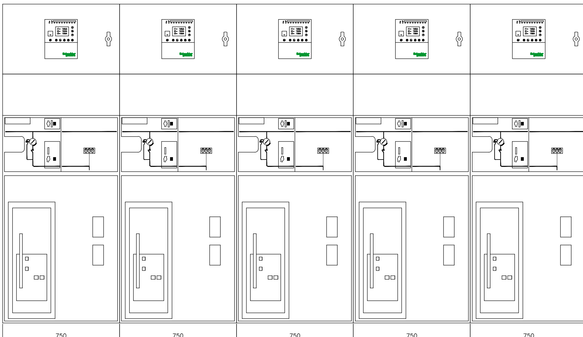
QMT-PU FRONTE QUADRO MEDIA TENSIONE PORT UTILITIES
