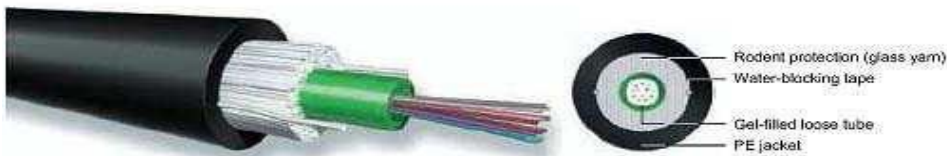
Figure 1: Fibre optic cable (cross section)
