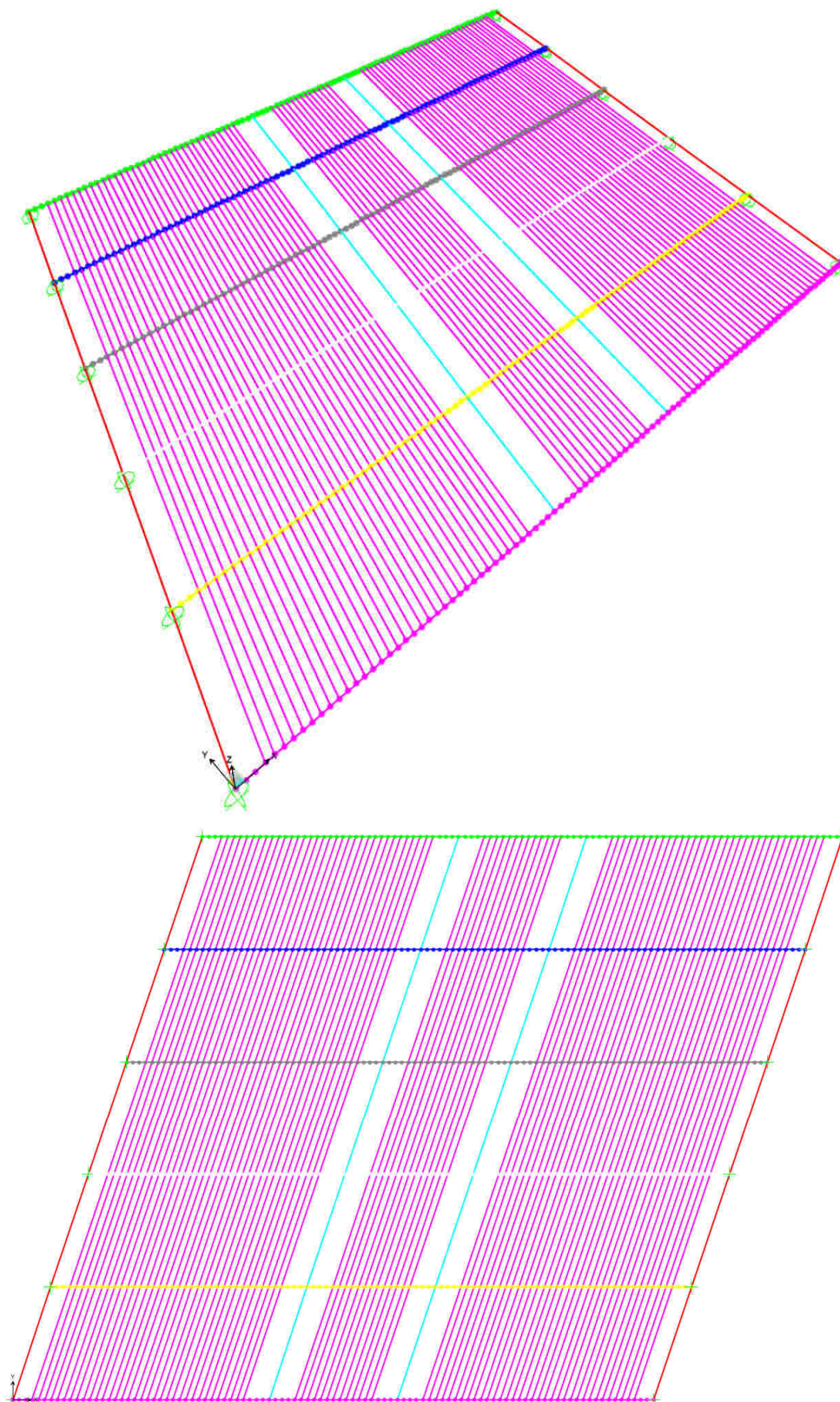
F 9. ST24 – Graticcio L = 16.35m a 6 Travi
