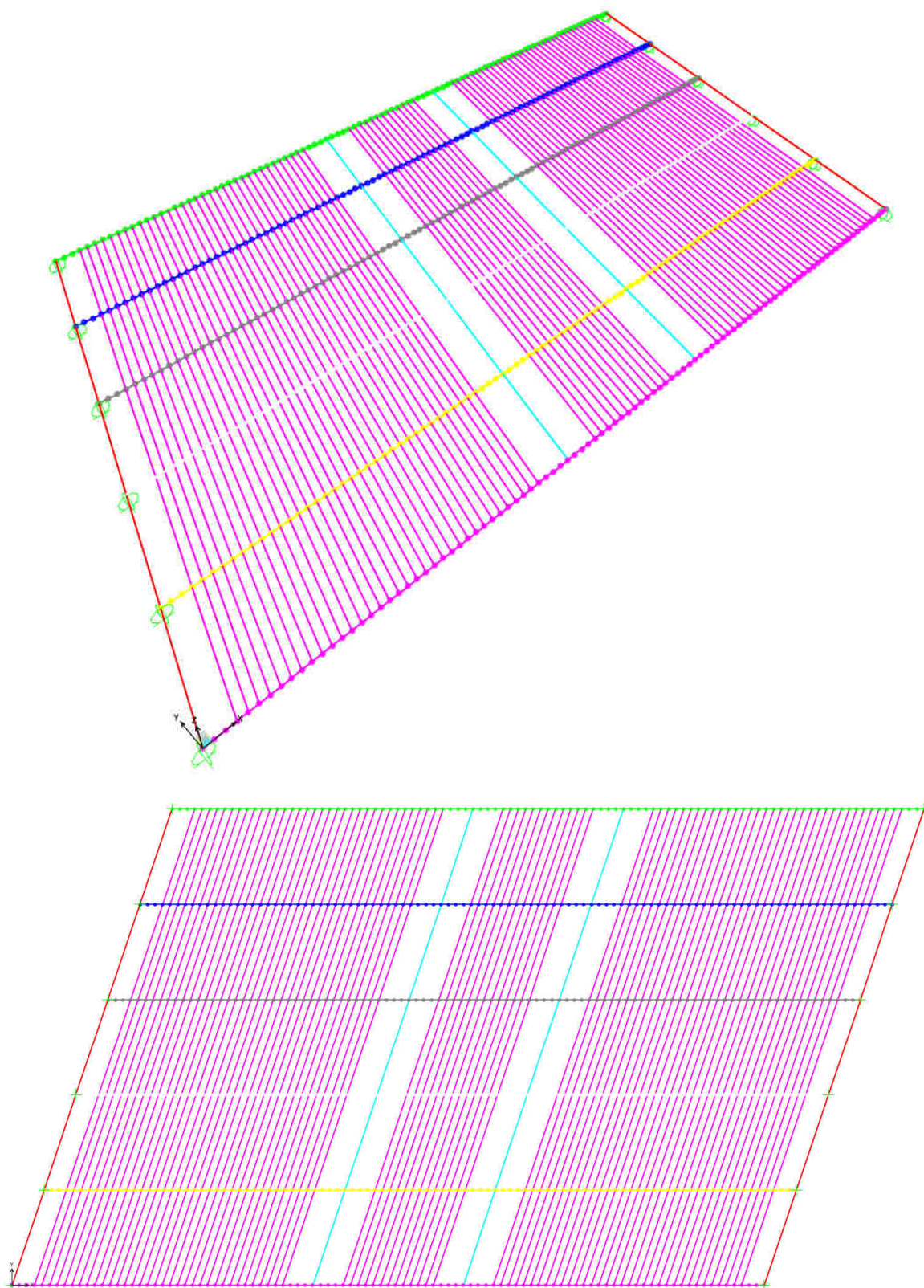
F 8. ST24 – Graticcio L = 22.70m a 6 Travi
