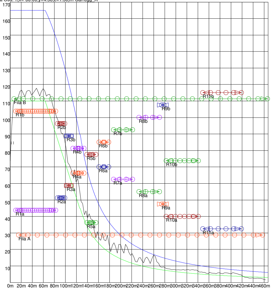
Luminanza Oss. 1(x=-60.00;y=4.58;z=1.50)m Carregg_A
