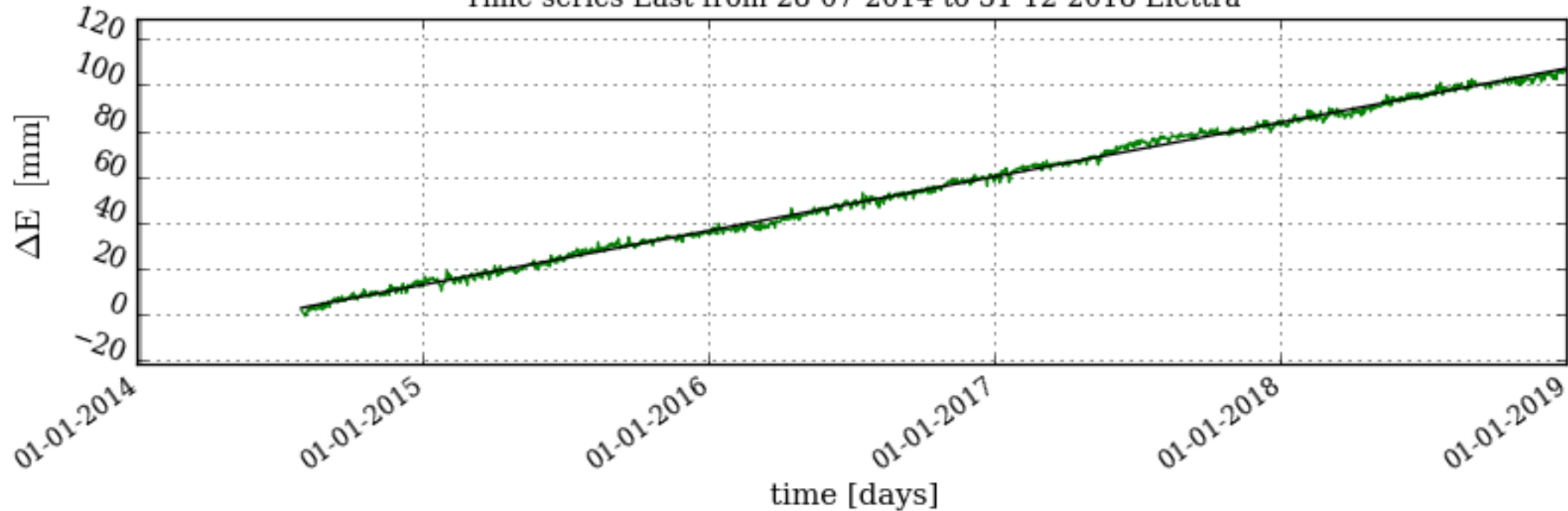
Time series East from 28-07-2014 to 31-12-2018 Elettra
