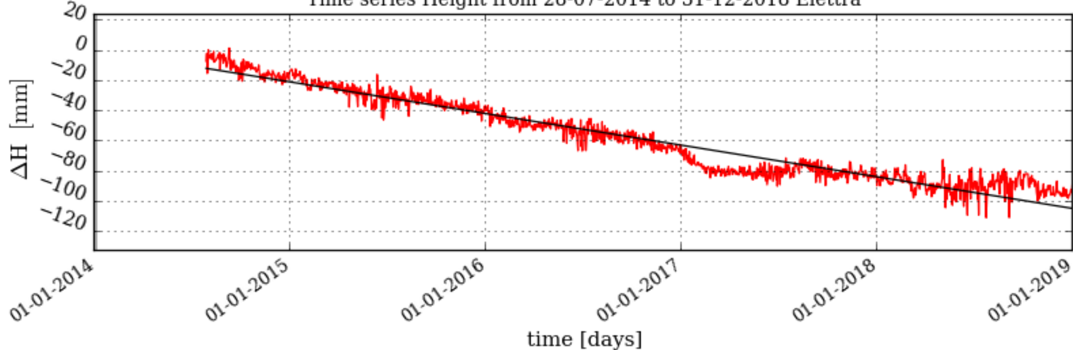
Time series Height from 28-07-2014 to 31-12-2018 Elettra
