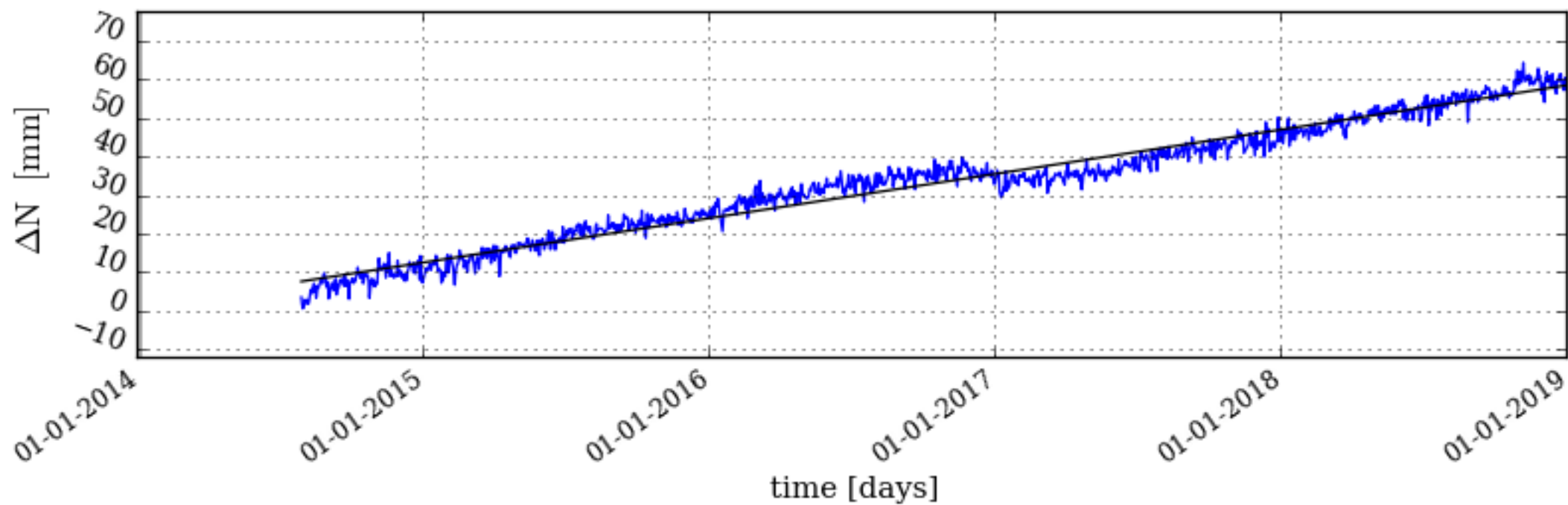
Time series North from 28-07-2014 to 31-12-2018 Elettra
