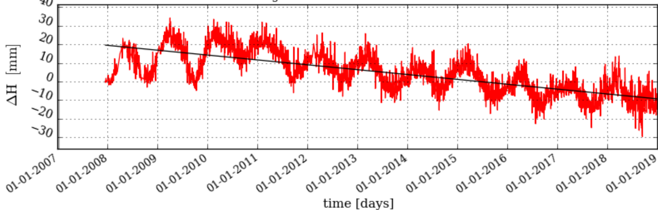
Time series Height from 13-12-2007 to 29-12-2018 Rubicone
