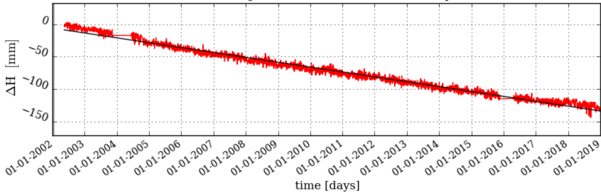
Time series Height from 07-05-2002 to 29-12-2018 Spinaroni
