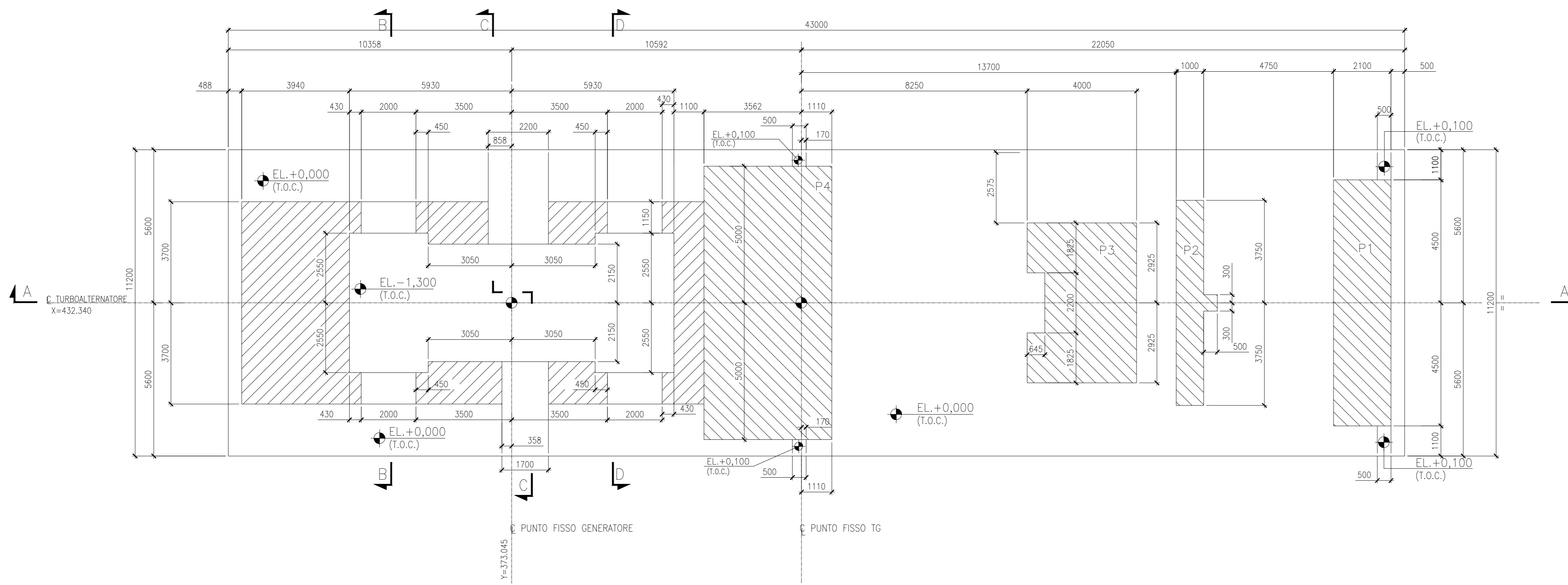
PIANTA EL. +0,000 SCALA 1:100
