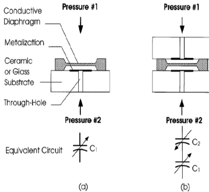
FIGURE 16.2 Operating principle of capacitive pressure sensors. (a) Single capacitor design; and (b) differential capacitor design.
