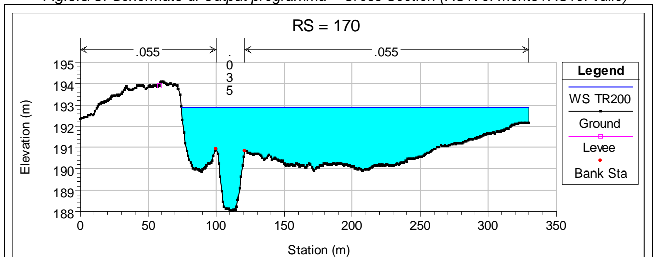
Fig.5.3/C: Schermate di Output programma – Cross Section (RS170: monte /RS10: valle)
