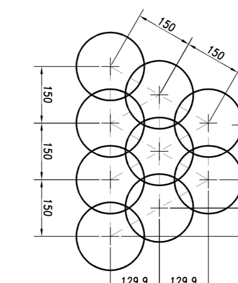
SCHEMA TAPPLO LFT-GROUTING Ø1800 scdia 1:100
