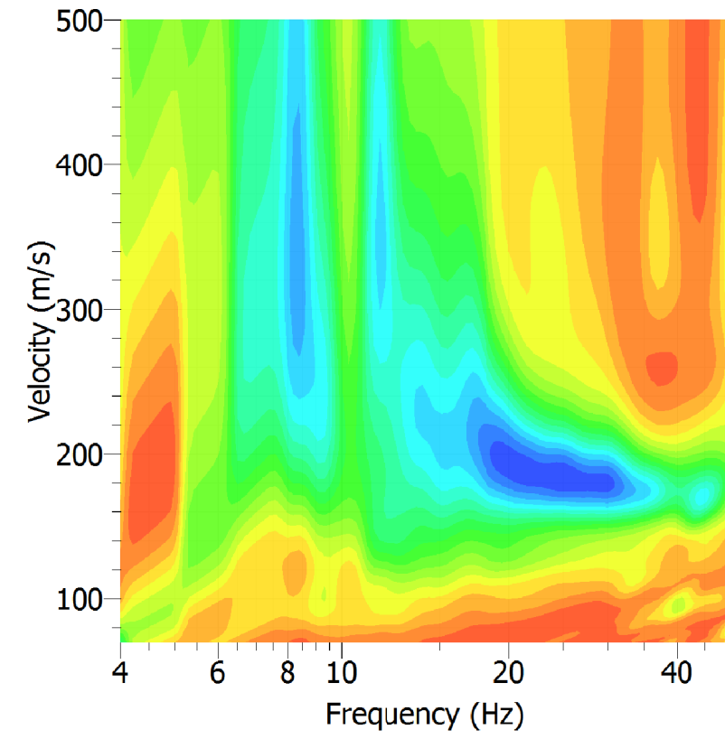
MASW 1 - Fortezza Dispersion curve - Rayleigh wave Shot at (-6, 0, 0)
