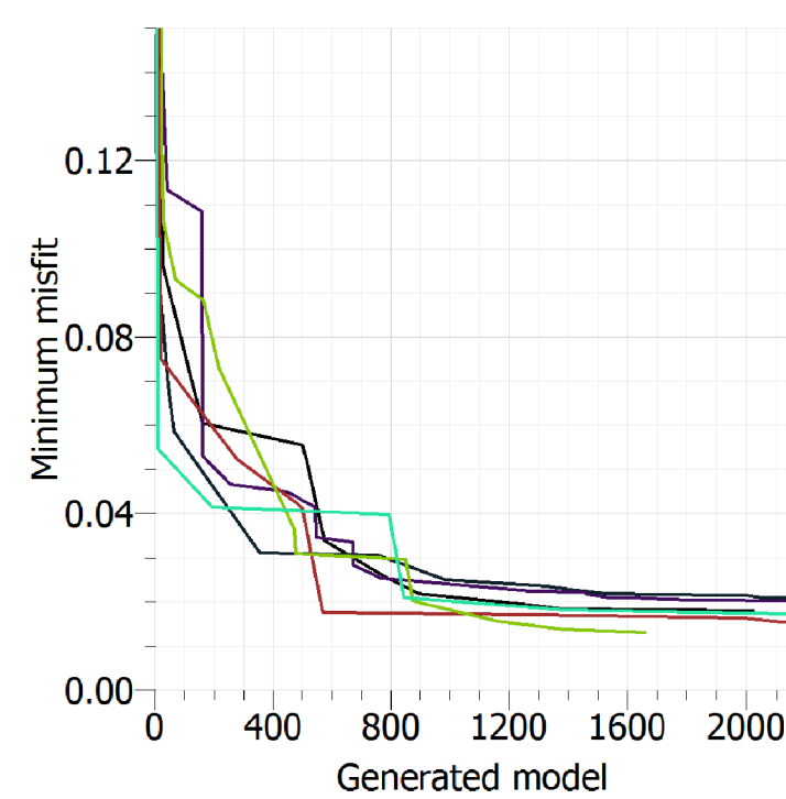
MASW misfit iteration model
