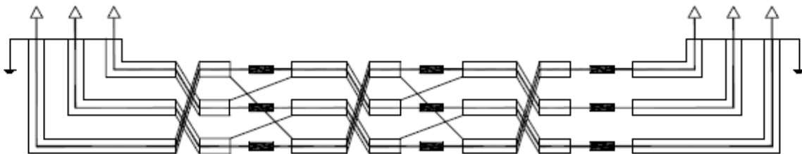
CROSS BONDING
