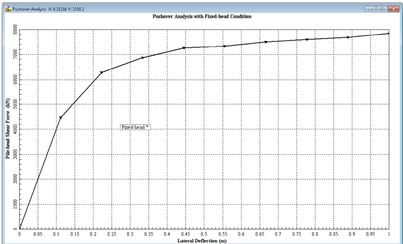
Figura 9-2: Analisi push-over palo
