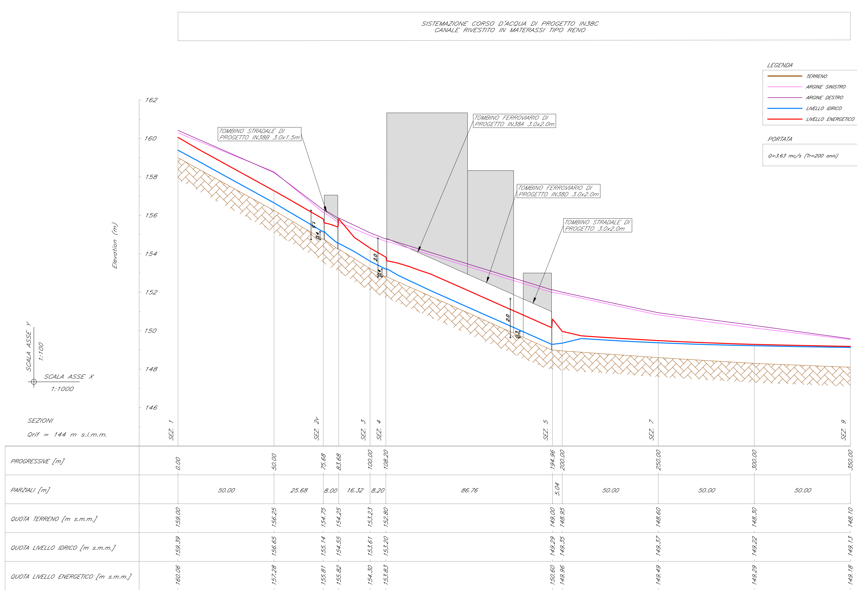
PROFILO POST OPERAM progr. 18+050
